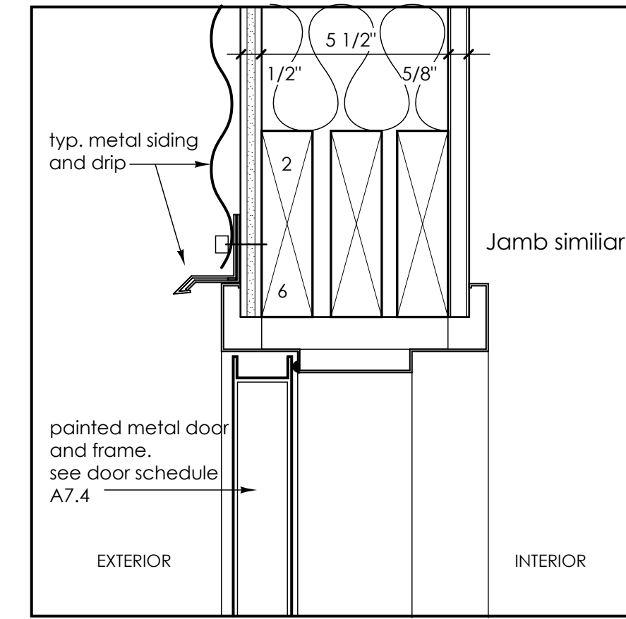
4 Head detail - roof egress stair at Courtyard Typ. Metal Frame @ Exterior 2x6 wall. 3"=1'-0"
