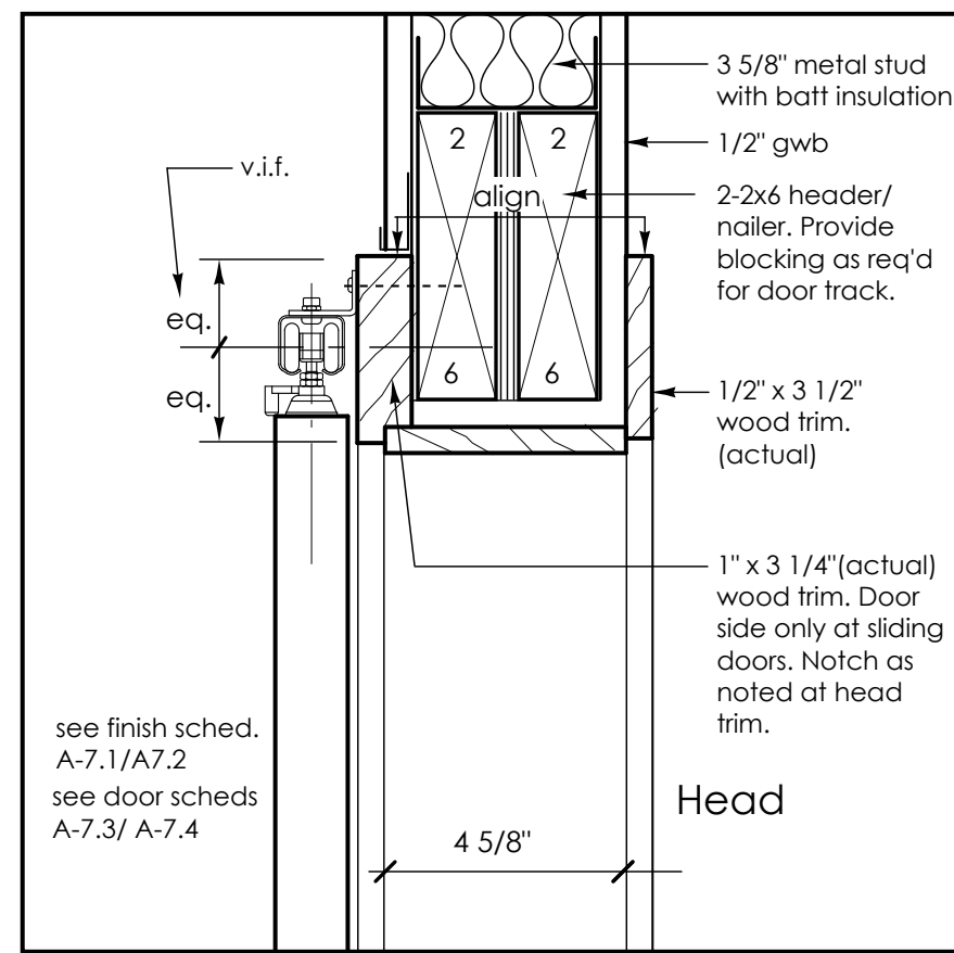
12 Head detail - interior sliding door 3"=1'-0"
