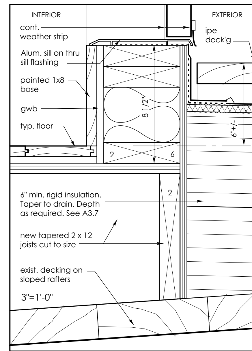
6 Sill detail - Free Street Mezzanine Roof Deck See 3/A3.7 adjacent window sill similar - see plan 3"=1'-0"
