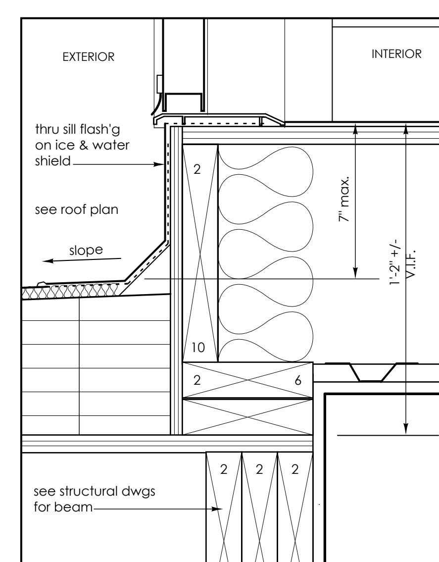
5 Sill detail - roof egress stair door 407A @ Courtyd 3"=1'-0" see A3.5 and A3.9
