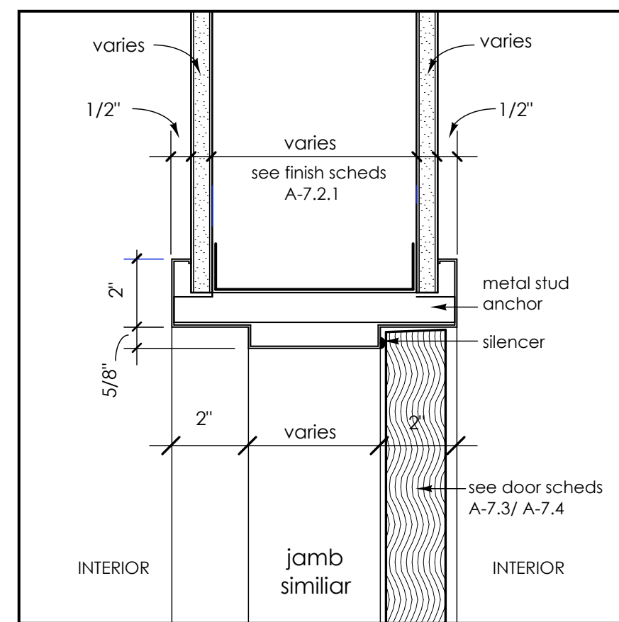
9 Typ. head detail - interior metal stud wall See A7.1 and A7.2 for wall types 3"=1'-0"
