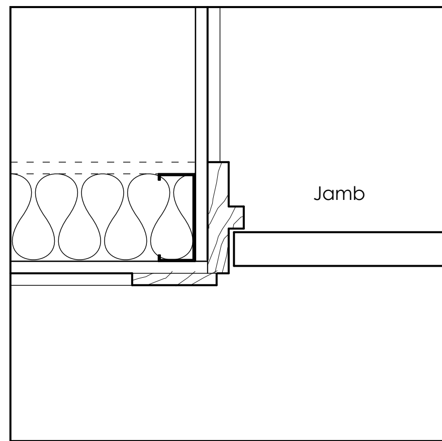
14 Jamb detail - interior sliding door 3"=1'-0"
