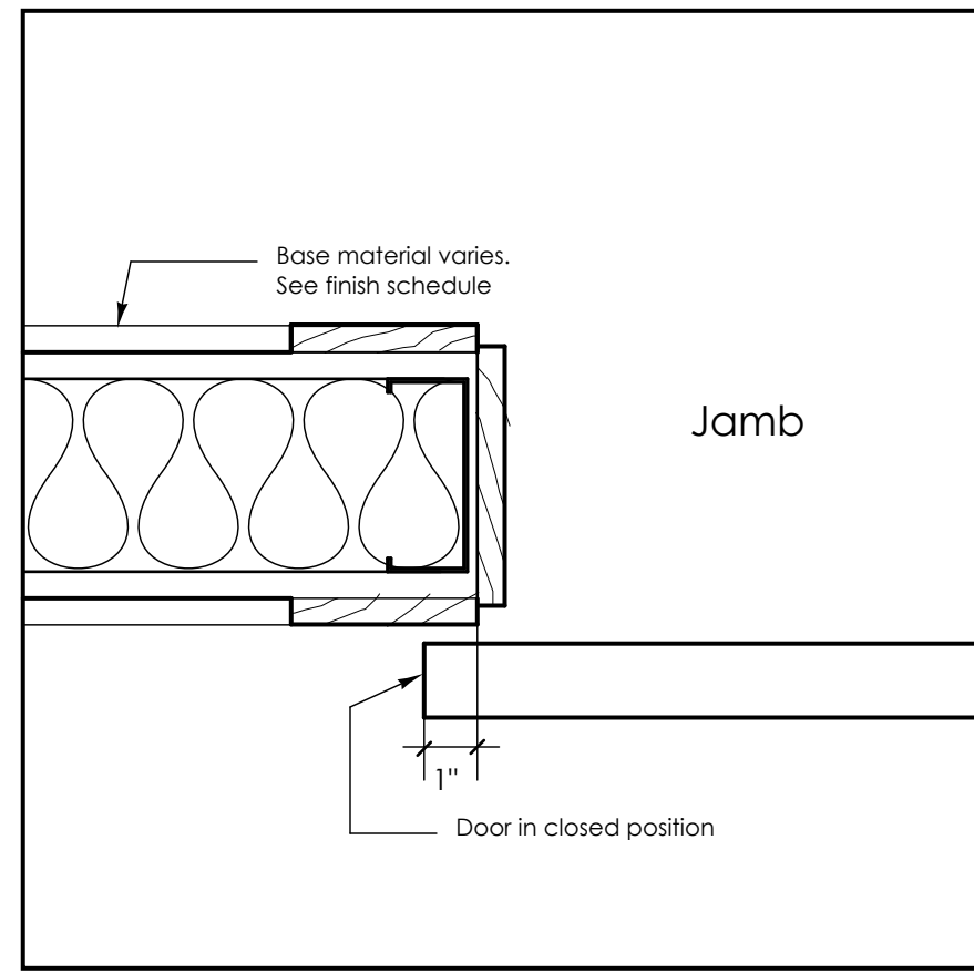
13 Jamb detail - interior sliding door 3"=1'-0"
