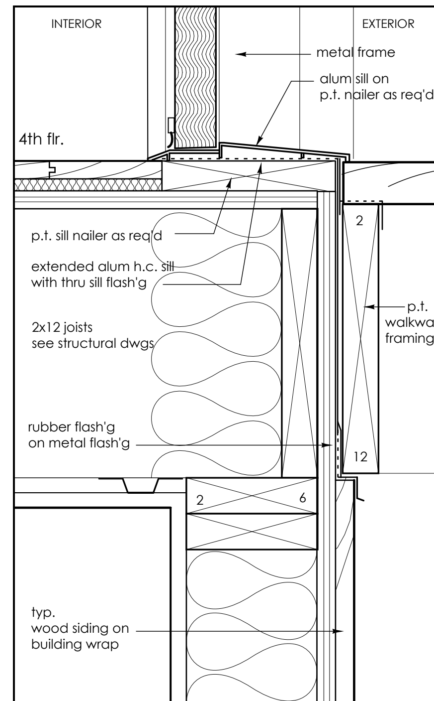
11 Sill detail - Congress St. bldg @ courtyard walkway See A3.8 3"=1'-0"
