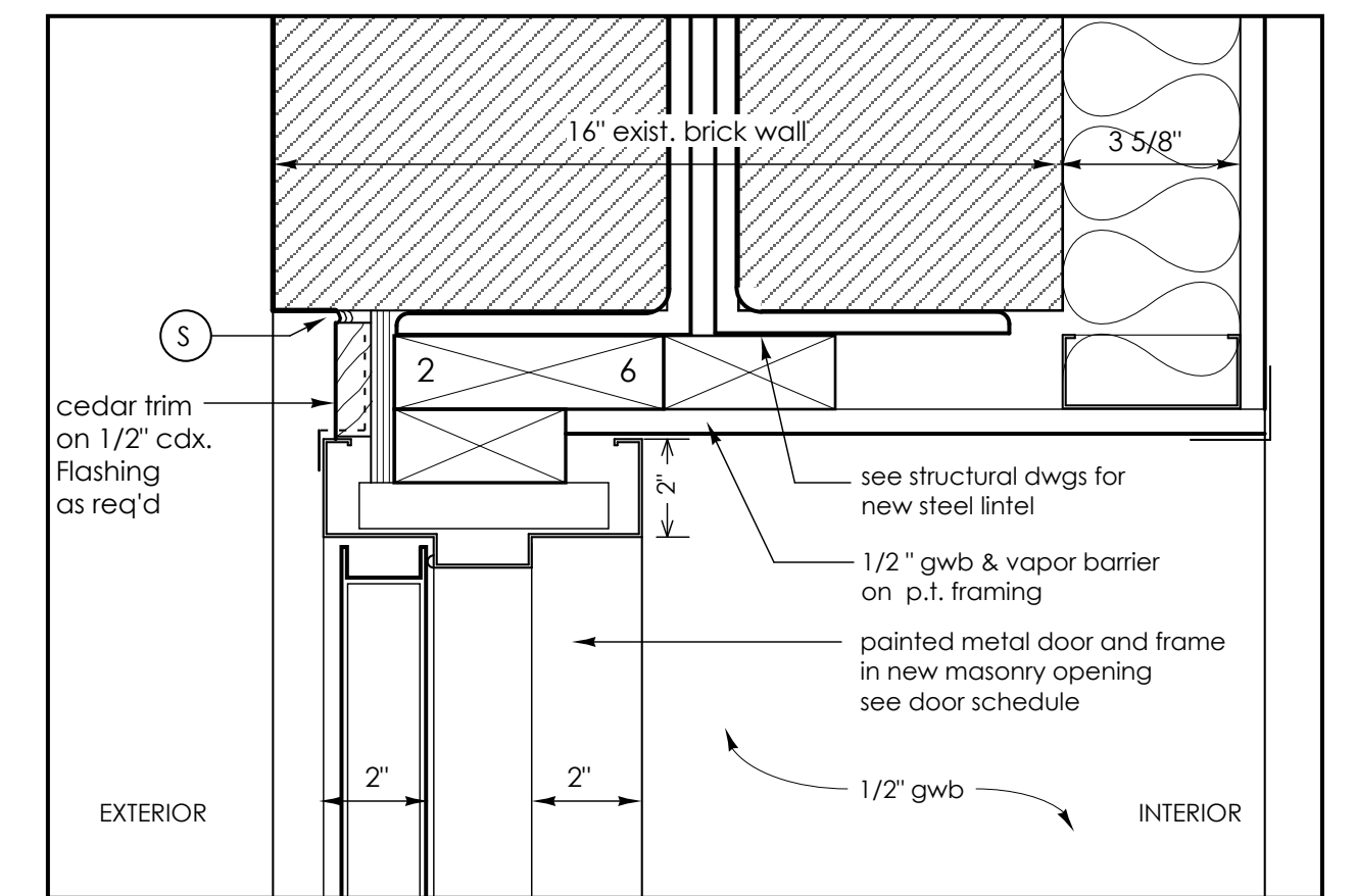
1 Head detail - free street exterior egress door 109B (jamb similar) 3"=1'-0"
