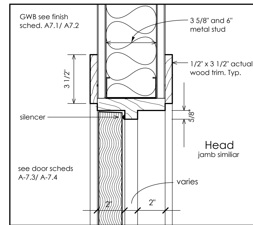
7 Head detail - typ. interior trim 3"=1'-0"
