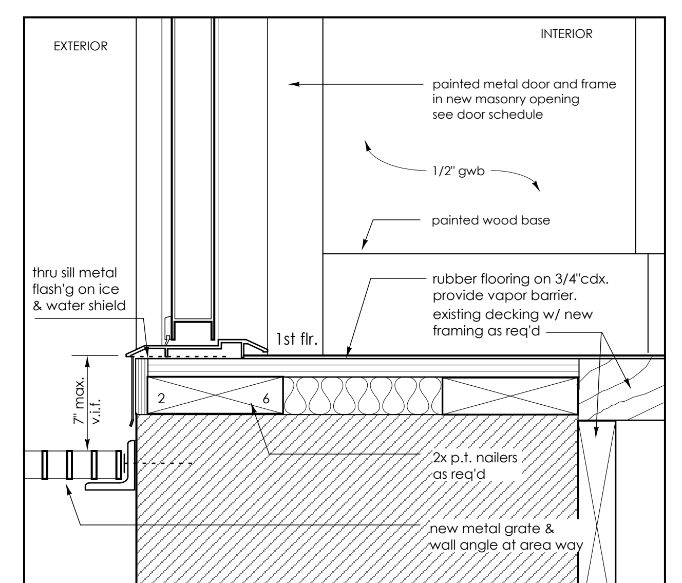
2 Sill detail - free street side exterior egress stair door 109B 3"=1'-0"
