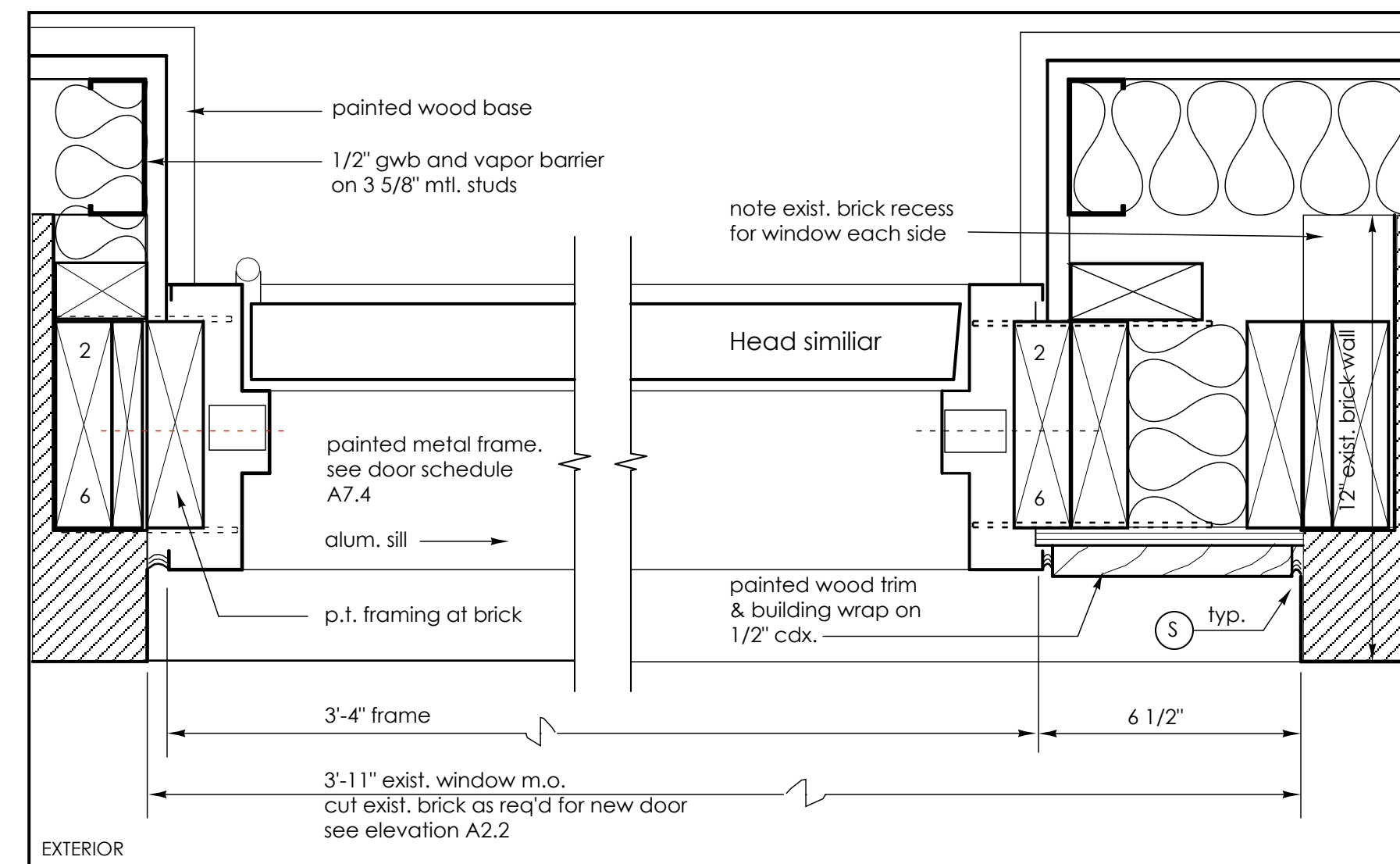
8 Jamb detail - free street courtyard @ new 3rd (305a) and 4th floor (405a) masonry opening. See 3 / A5.1 for sill 3"=1'-0"
