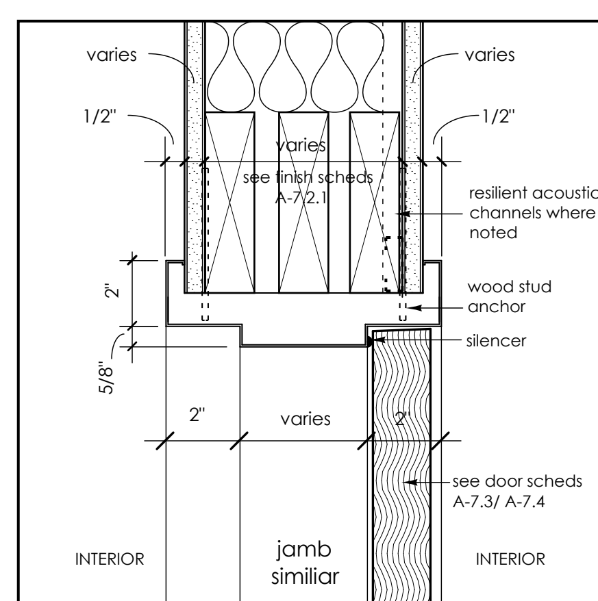
10 Typ. head detail - interior wood stud wall See A7.1 and A7.2 for wall types 3"=1'-0"
