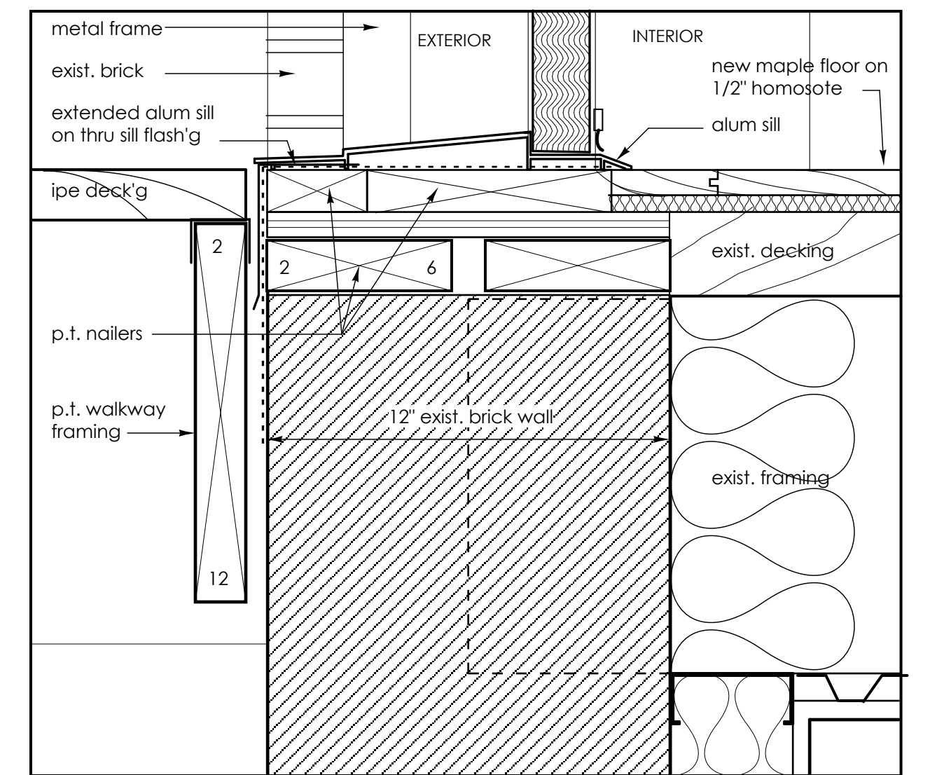
3 Sill detail - free street courtyard @ new 3rd (305a) and 4th floor (405a) masonry opening. 3"=1'-0"
