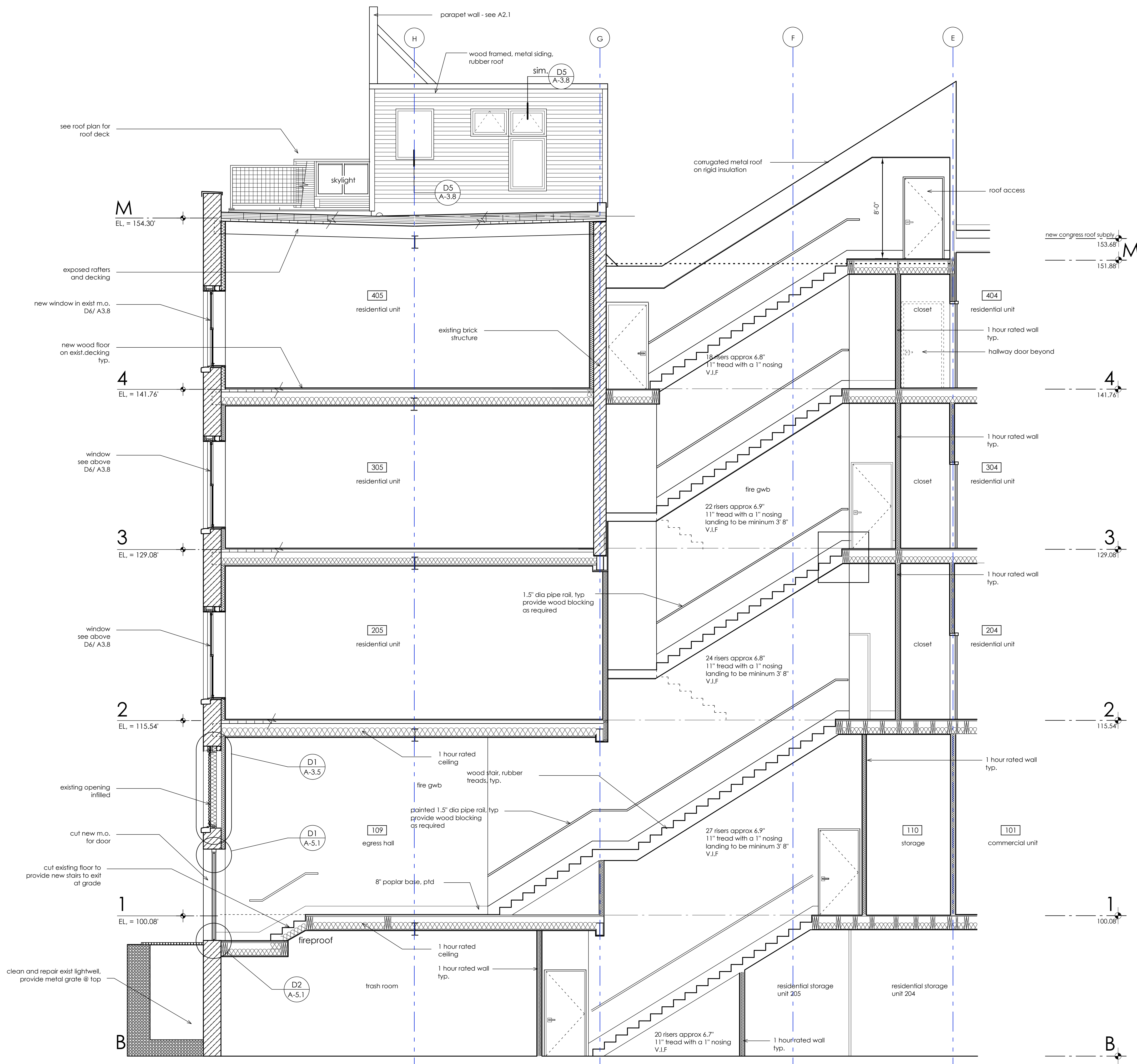
1 free street stair section detail
