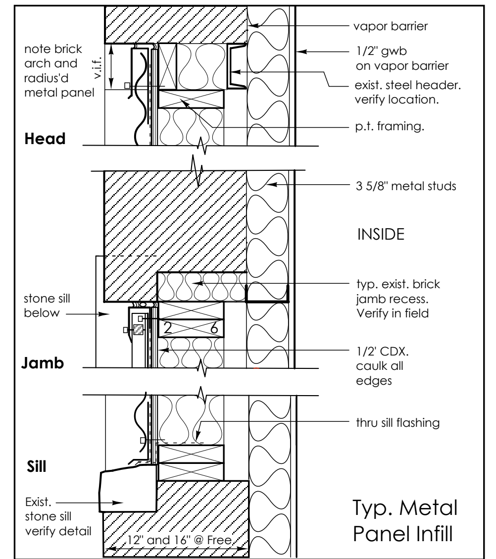
1 Detail - Metal panel at exist. Free Street window 3" = 1'-0" See A-2.1
