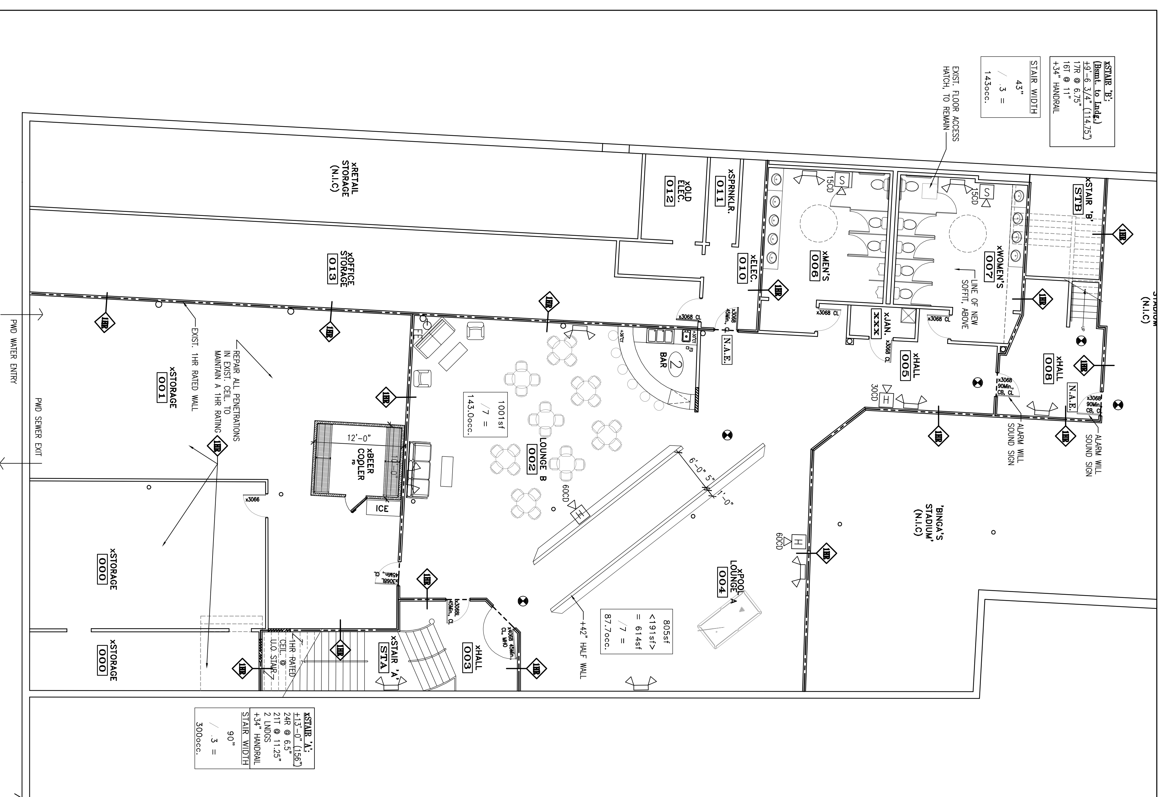
LIFE SAFETY BASEMENT PLAN SCALE: 1/8" = 1'-0"
