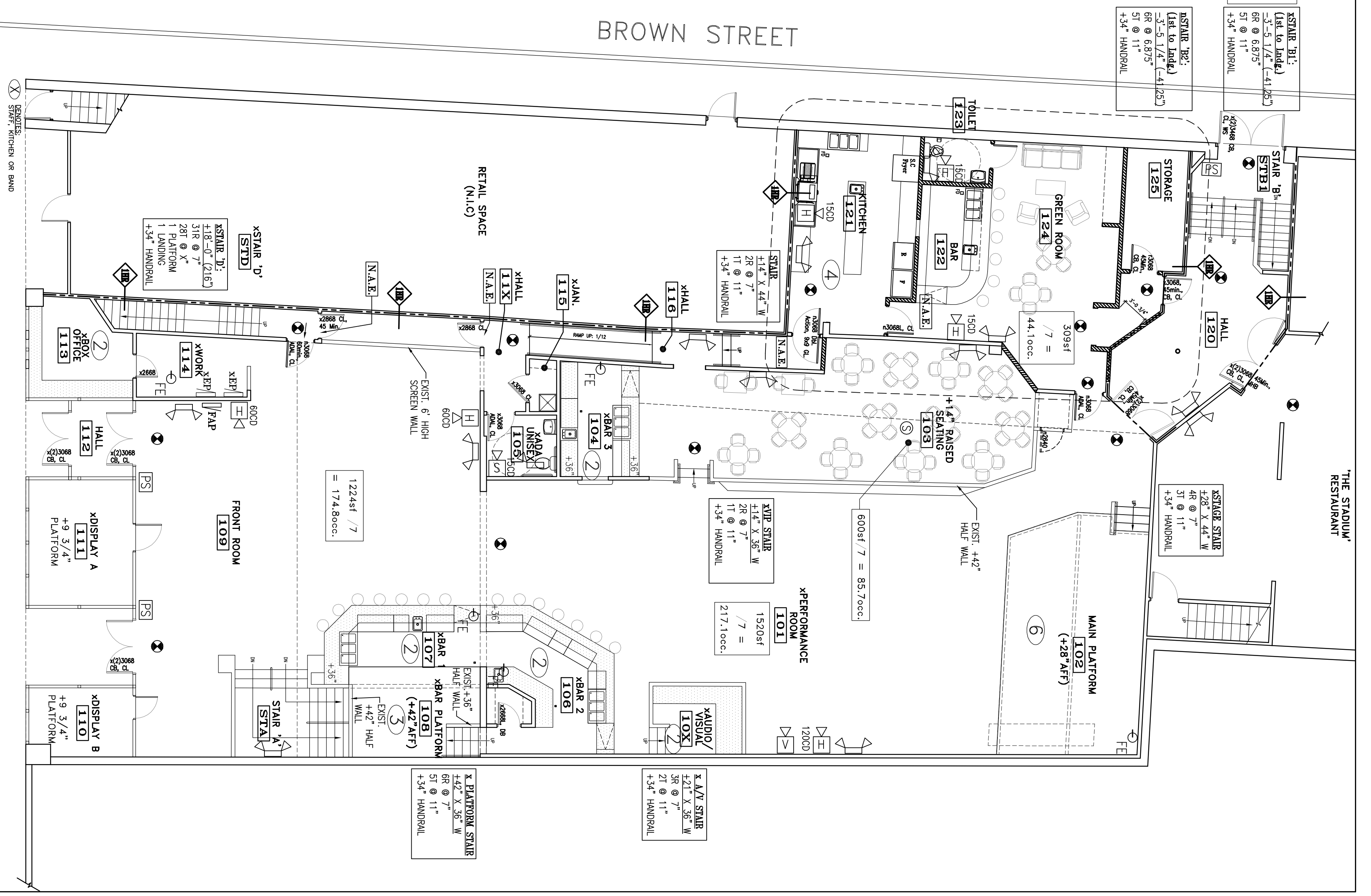
LIFE SAFETY FIRST FLOOR PLAN SCALE: 1/8" = 1'-0"
