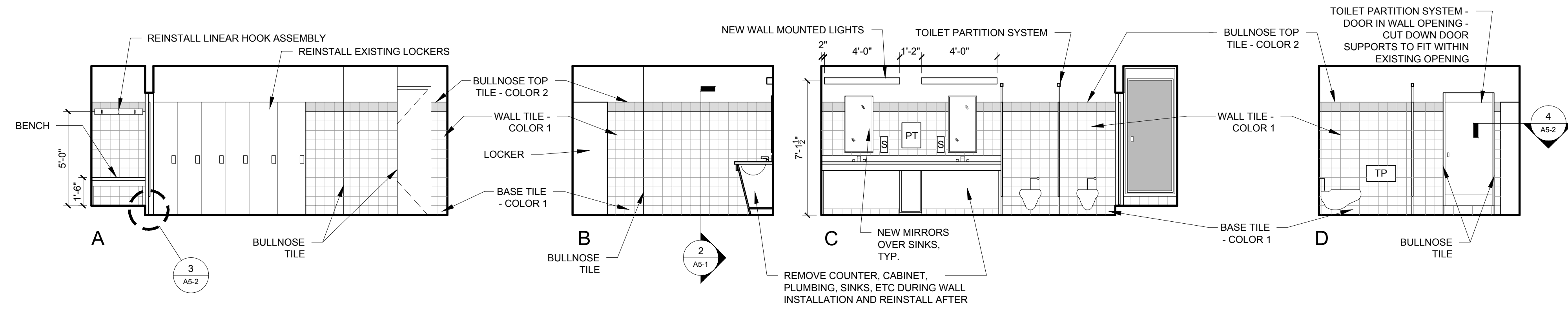
1 WOMENS LOCKER ROOM # 302 1/4" = 1'-0"
