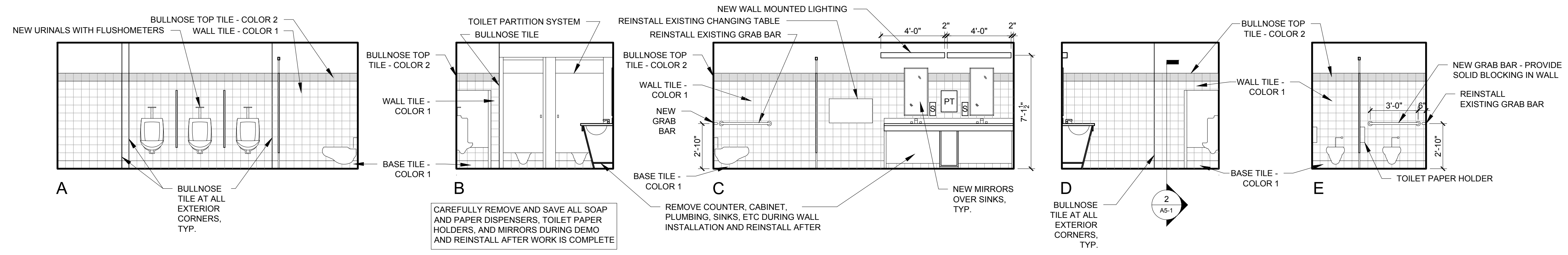
3 MENS LAV # 312 1/4" = 1'-0"
