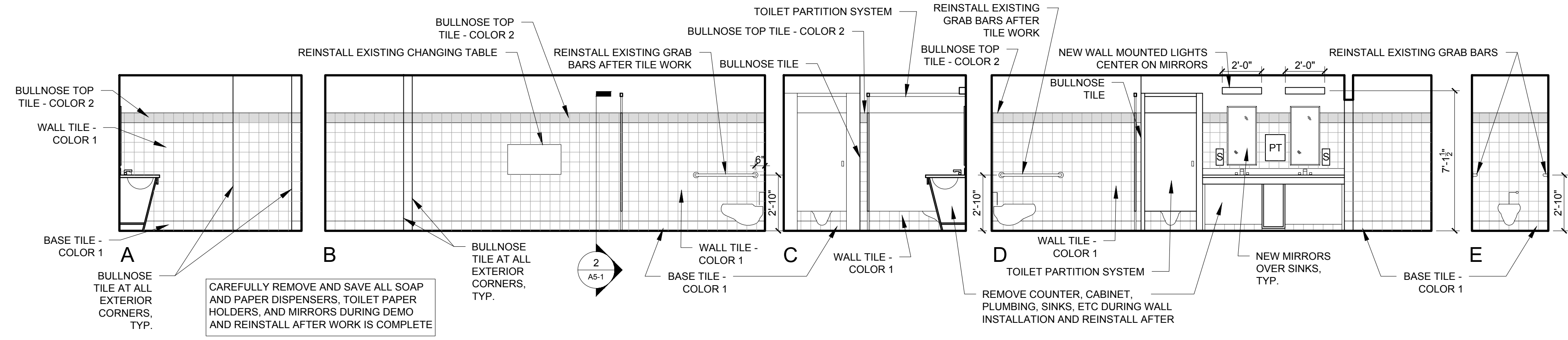
4 WOMENS LAV # 310 1/4" = 1'-0"
