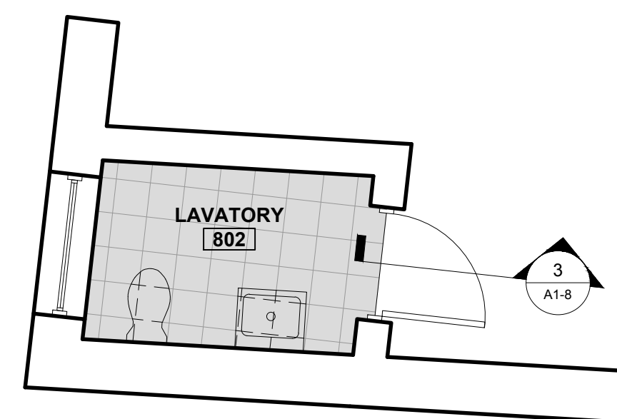
2 LAVATORY #802 1/4" = 1'-0"
