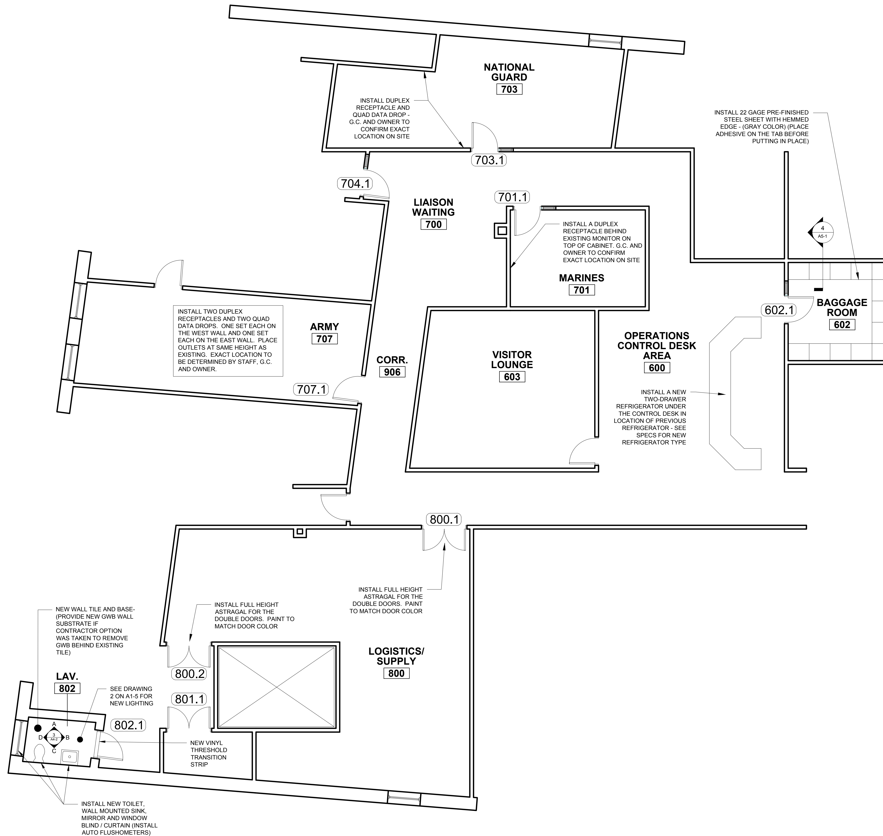
1 OPERATIONS FLOOR PLAN 3/16" = 1'-0"
