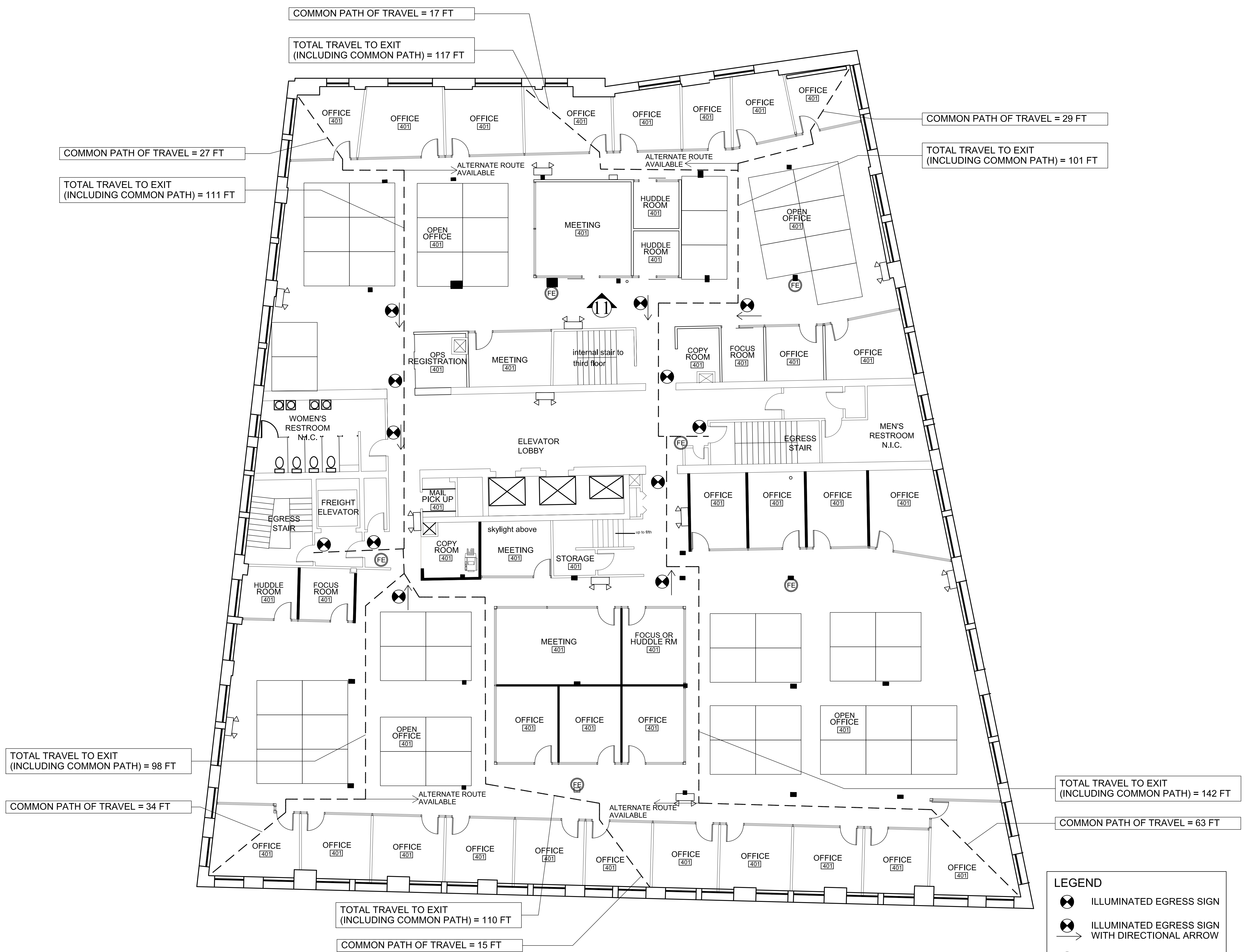
1 | 4TH FLOOR PLAN SCALE: 1/8" = 1'-0"
