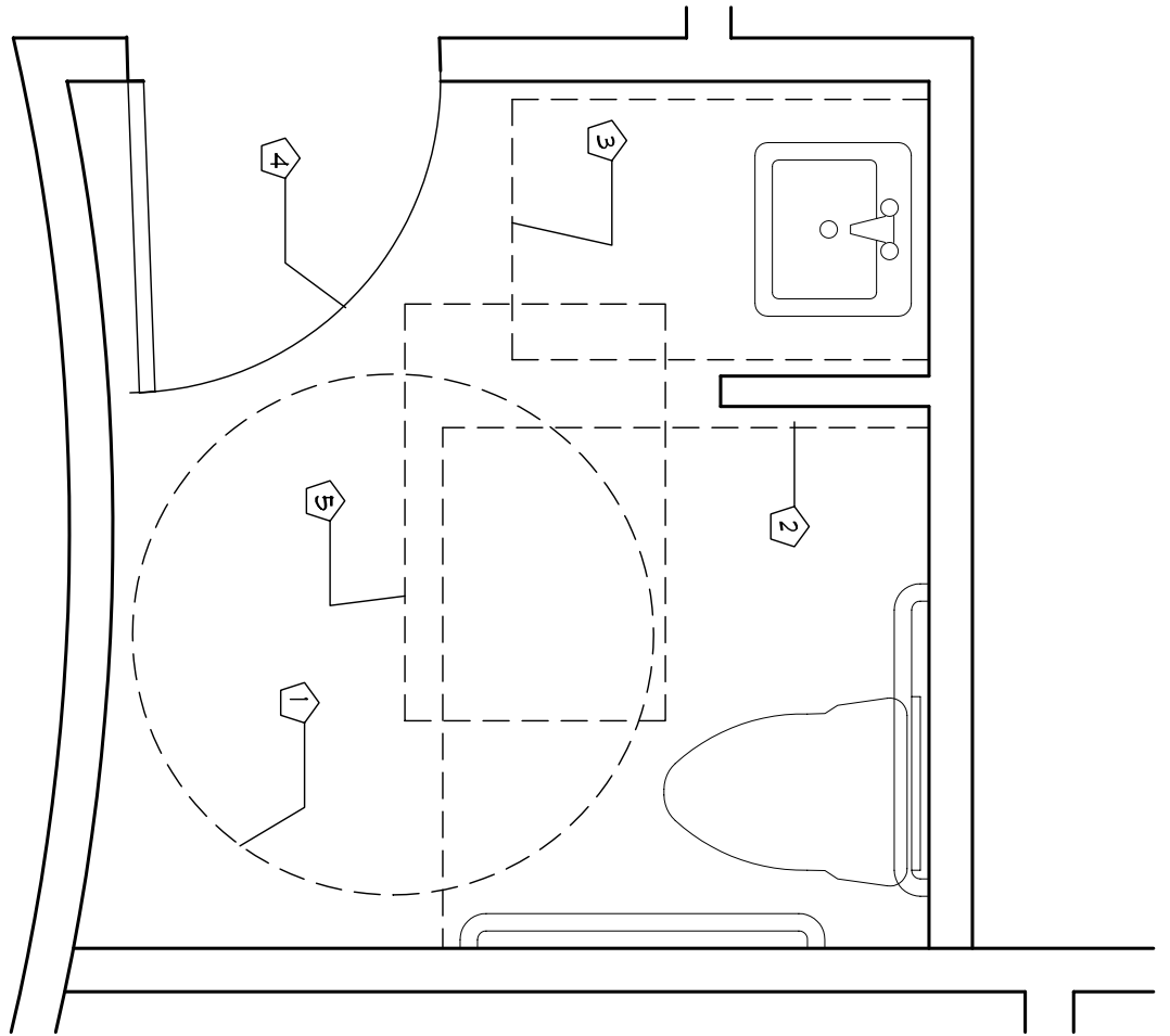
1 ADA BATHROOM PLAN SCALE: 1/2" = 1'-0"
