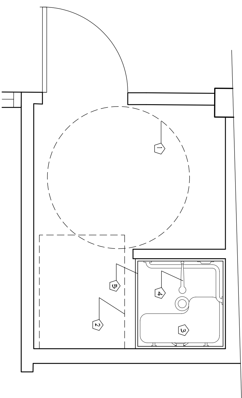
2 ADA SHOWER PLAN SCALE: 1/2" = 1'-0"
