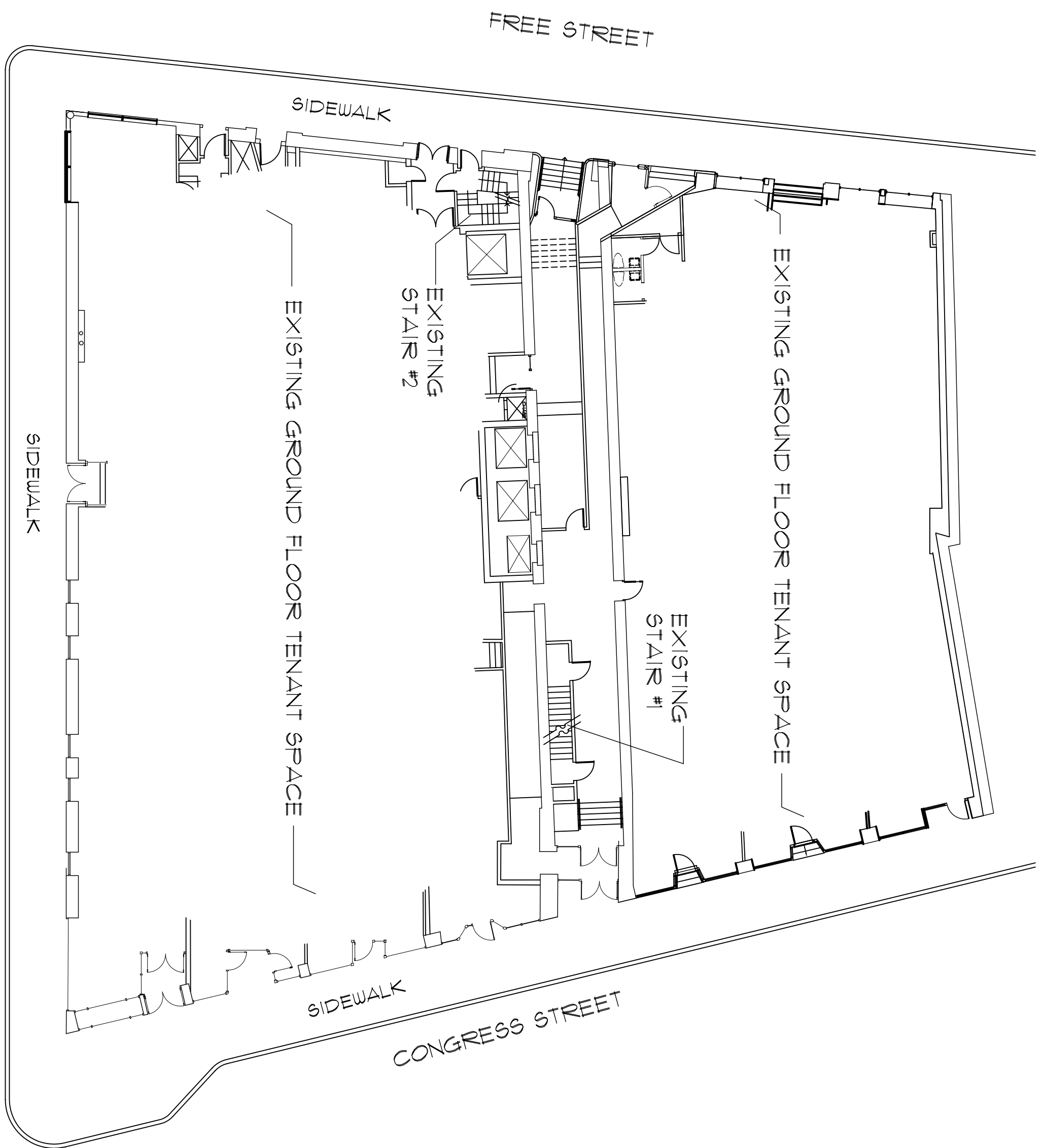
4 GROUND FLOOR EGRESS PLAN SCALE: 1/16" = 1'-0"
