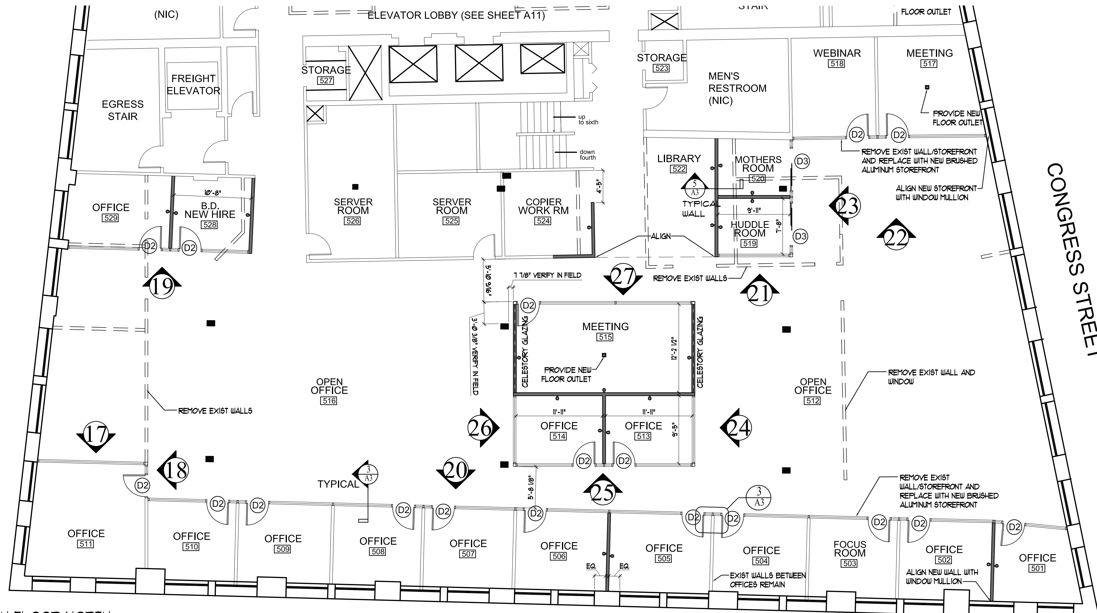
1 FLOOR PLAN - 5TH FLOOR NORTH SCALE: 1/8"=1'-0"
