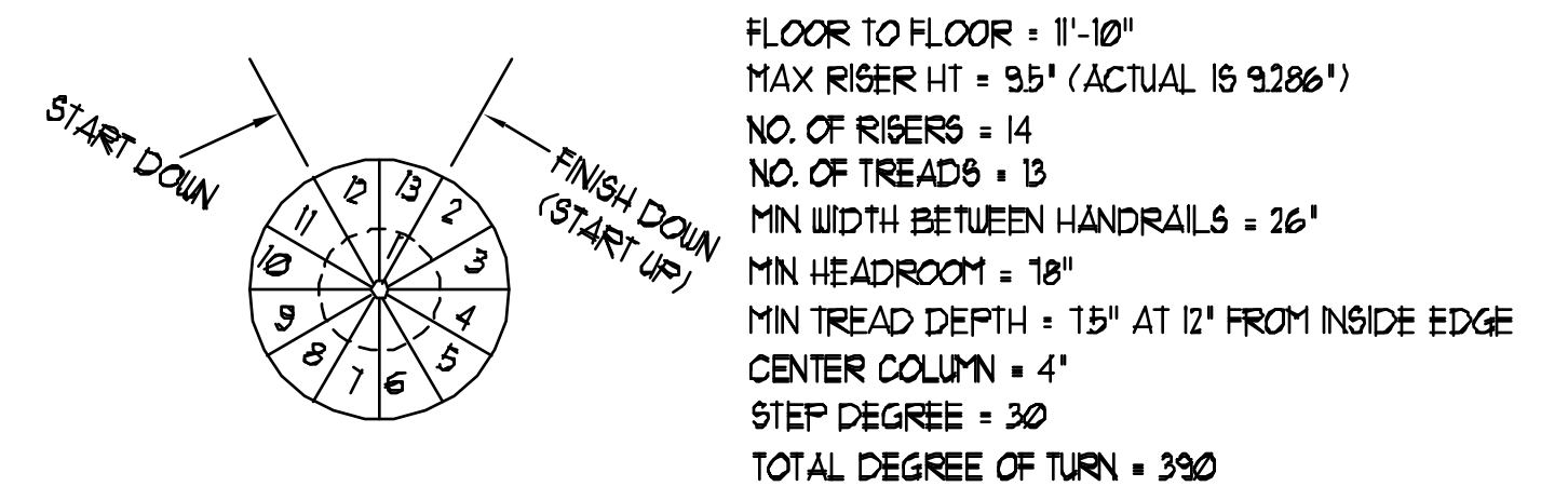
2 SPIRAL STAIR DETAILS (584 CONGRESS) SCALE: NTS
