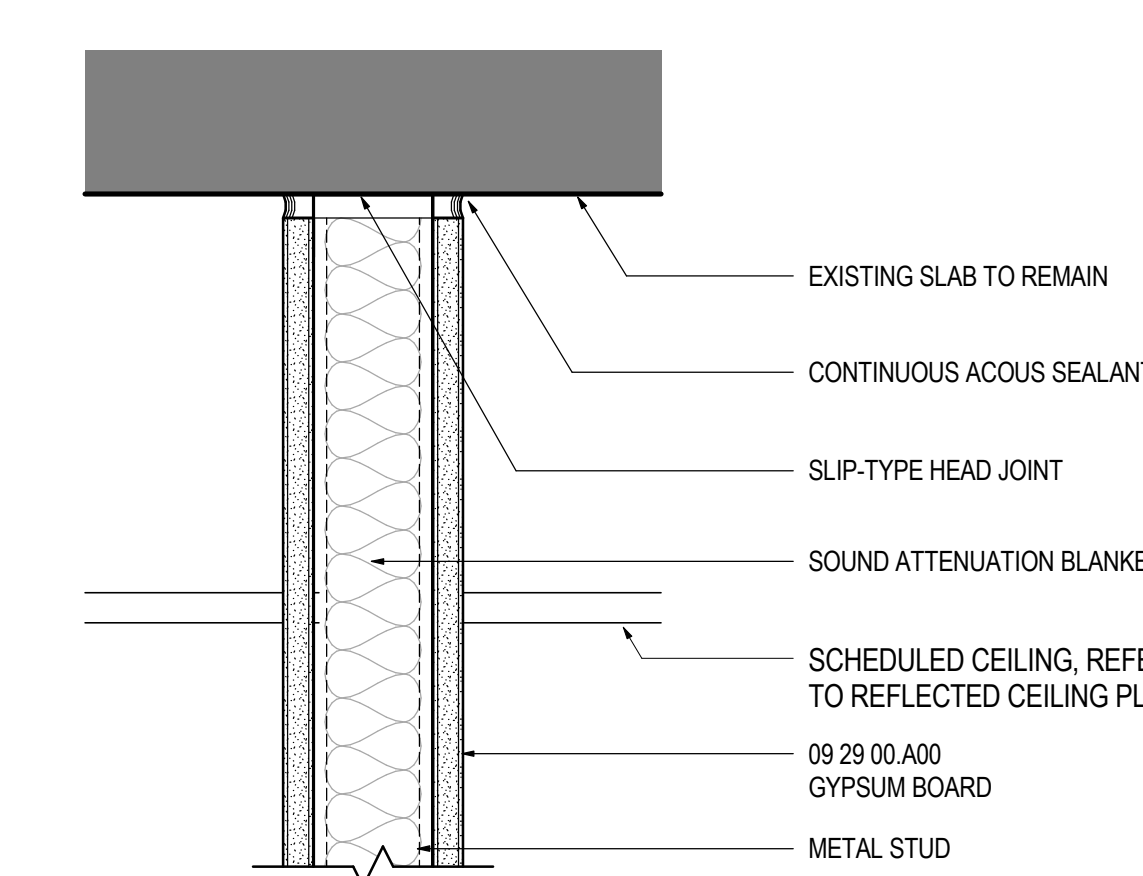
PARTITION HEAD DETAIL A-T04
