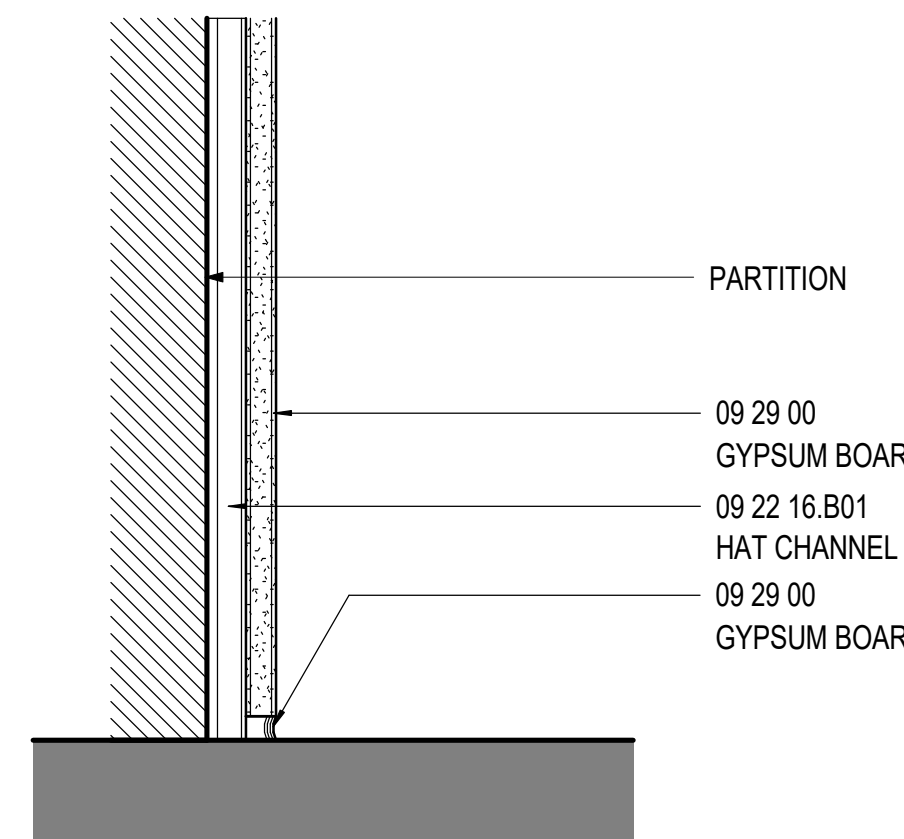
PARTITION BASE DETAIL F-B01
