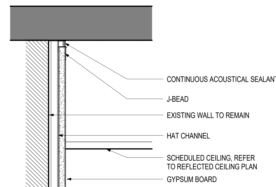
PARTITION HEAD DETAIL F-T04
