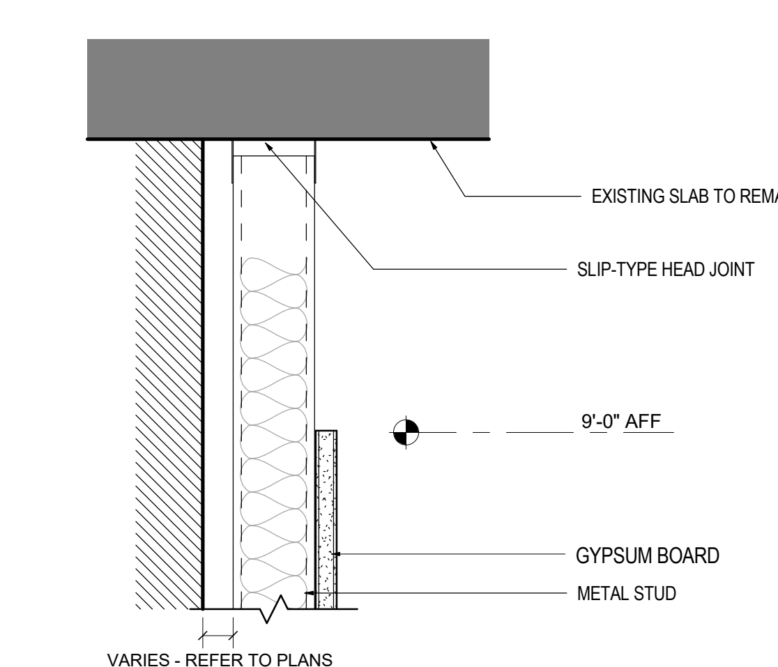
PARTITION HEAD DETAIL D-T05
