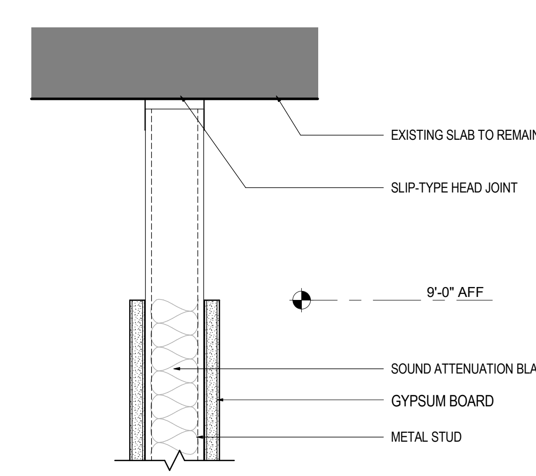
PARTITION HEAD DETAIL A-T05
