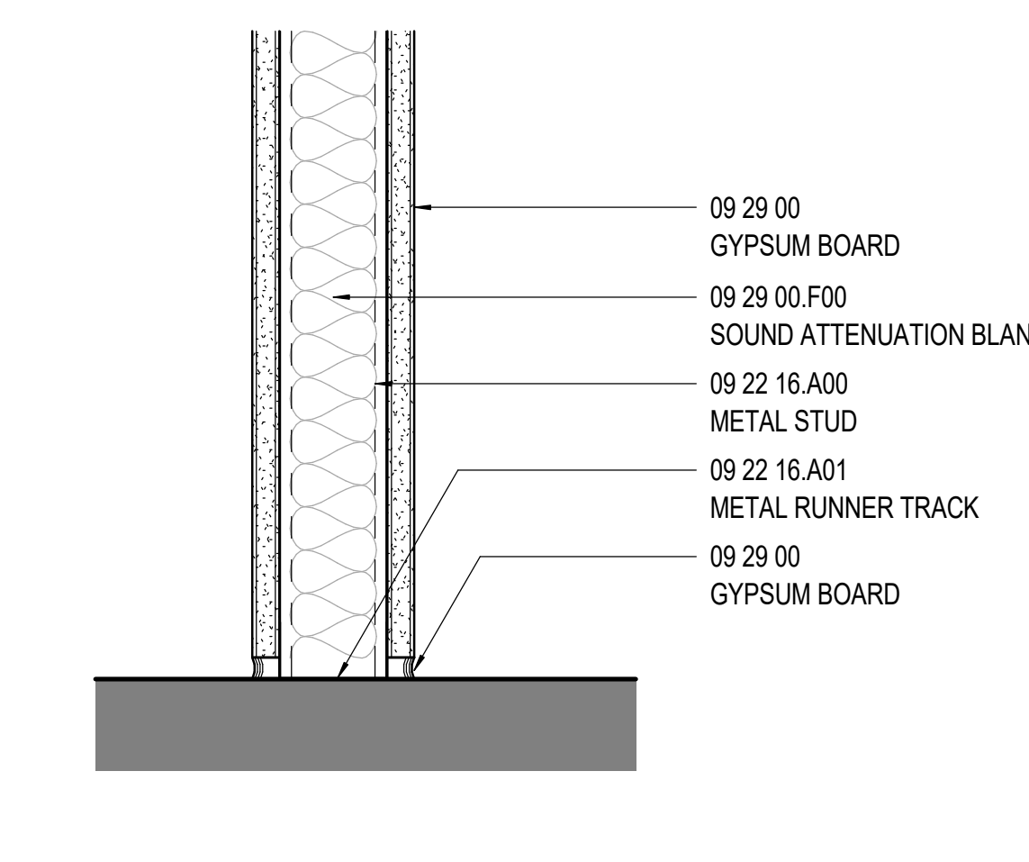
PARTITION BASE DETAIL A-B01
