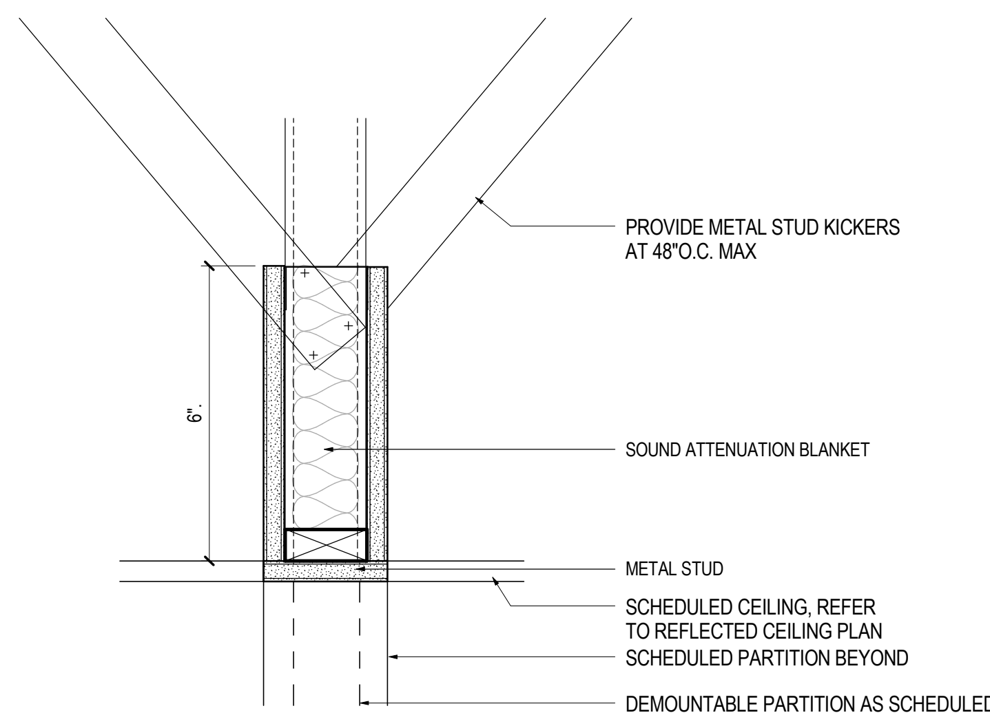
PARTITION HEAD DETAIL Q-T01
