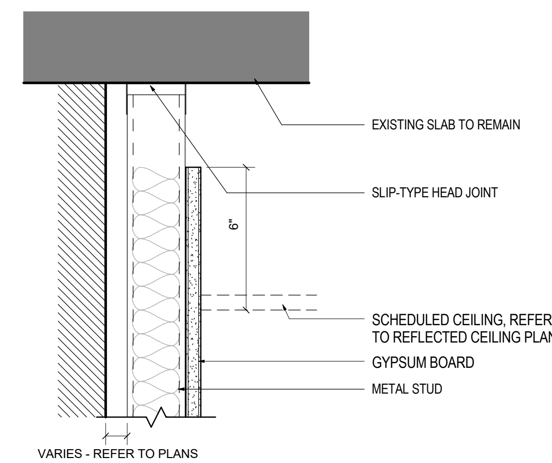
PARTITION HEAD DETAIL D-T01
