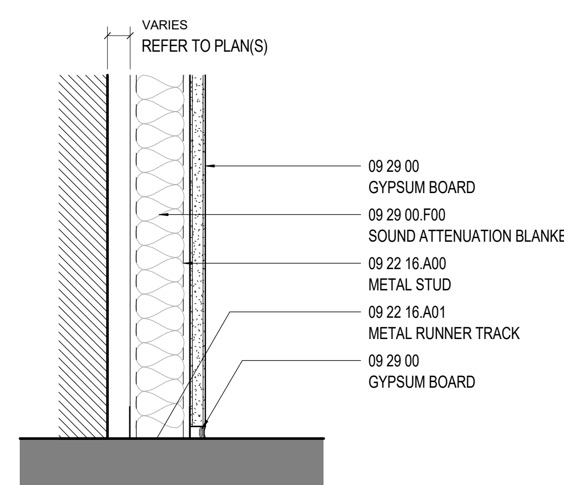
PARTITION BASE DETAIL D-B01
