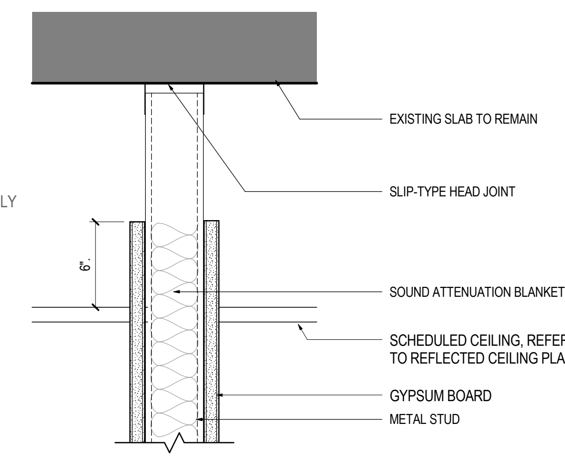
PARTITION HEAD DETAIL A-T02
