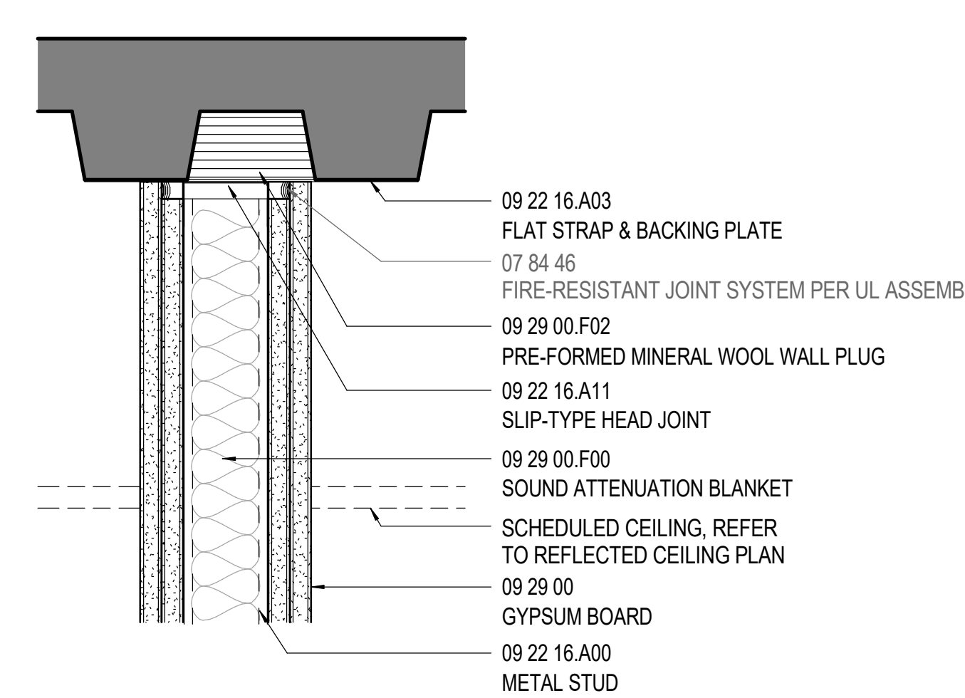
PARTITION HEAD DETAIL B-T01
