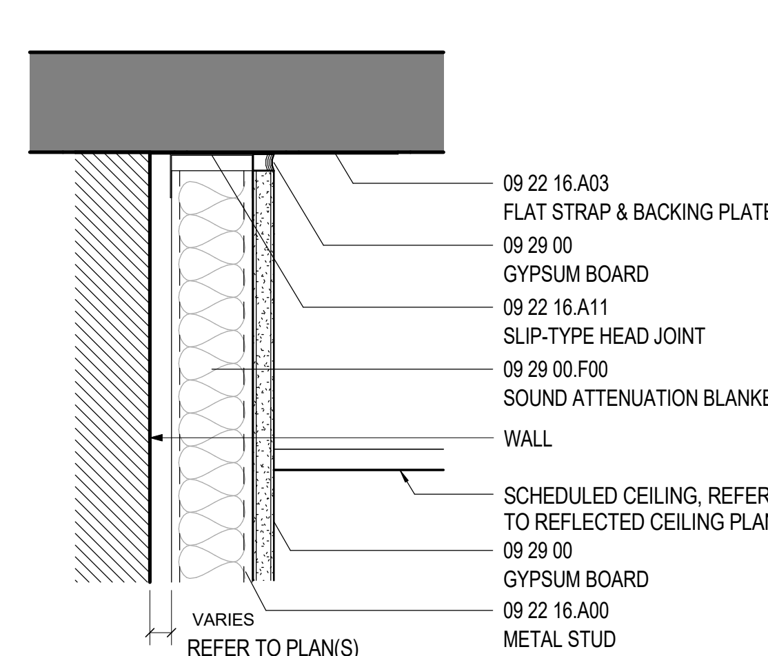
PARTITION HEAD DETAIL D-T04
