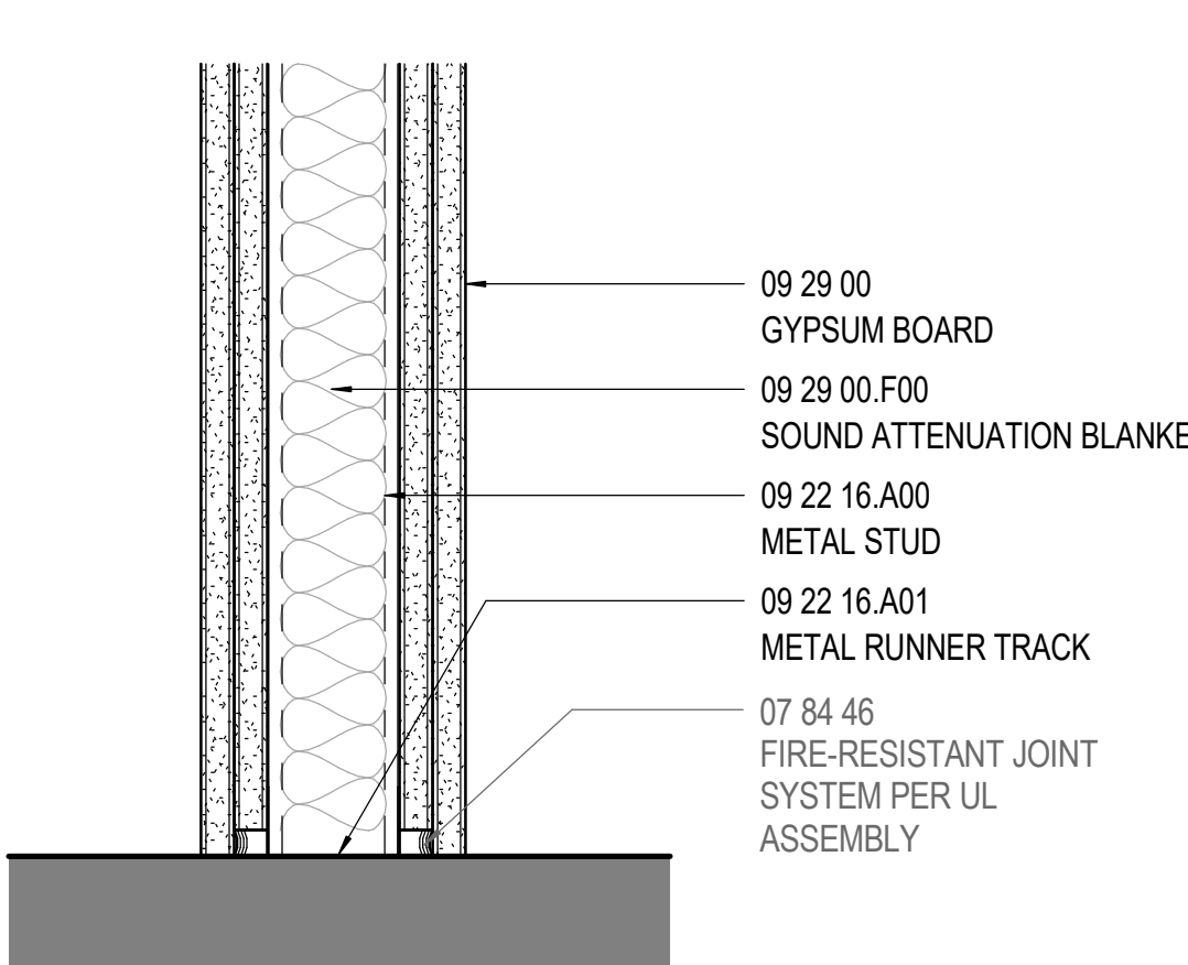
PARTITION BASE DETAIL B-B01
