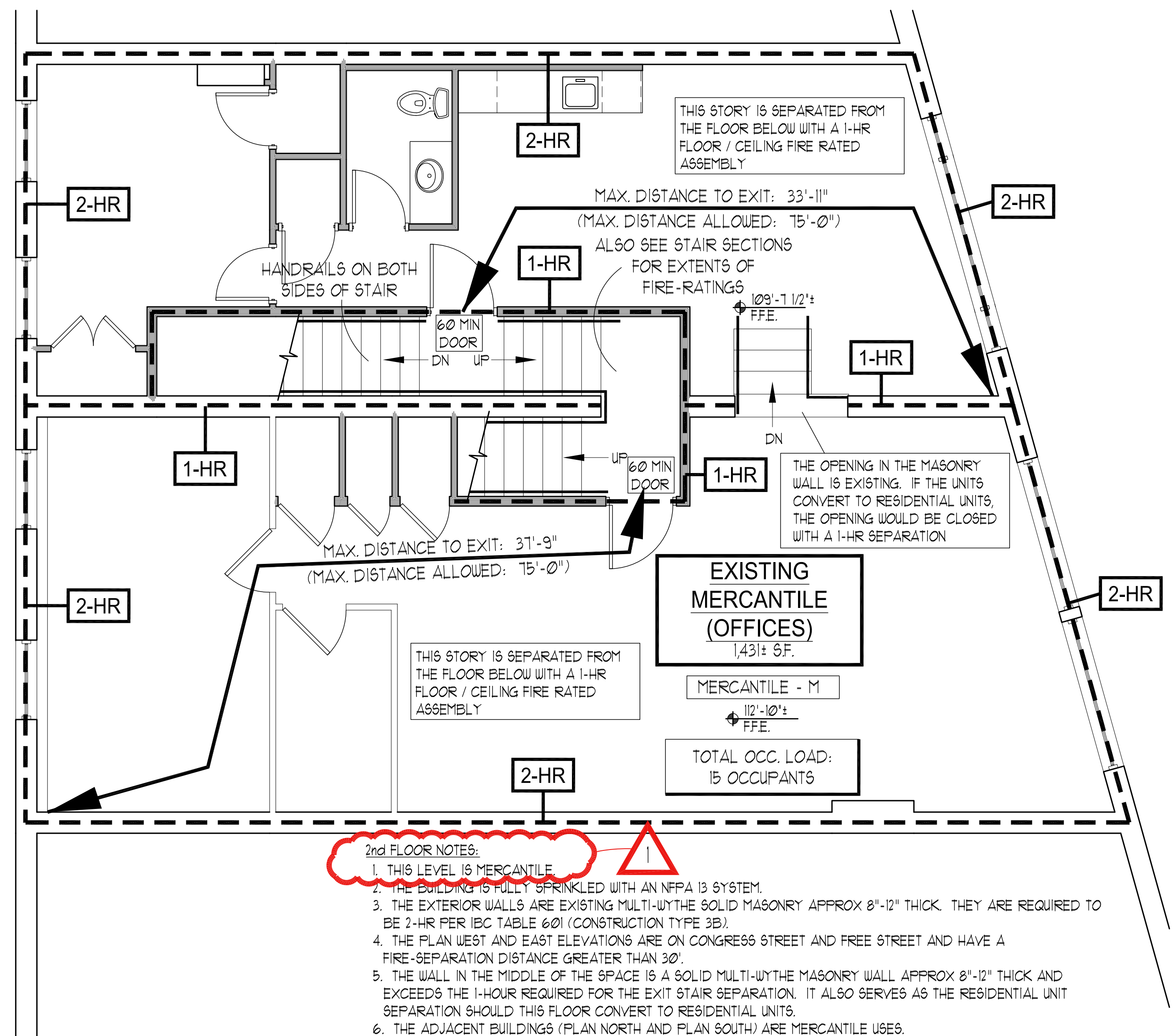
2 2nd FLOOR EGRESS PLAN - 582 & 584 SCALE: 1/4" = 1'-0"
