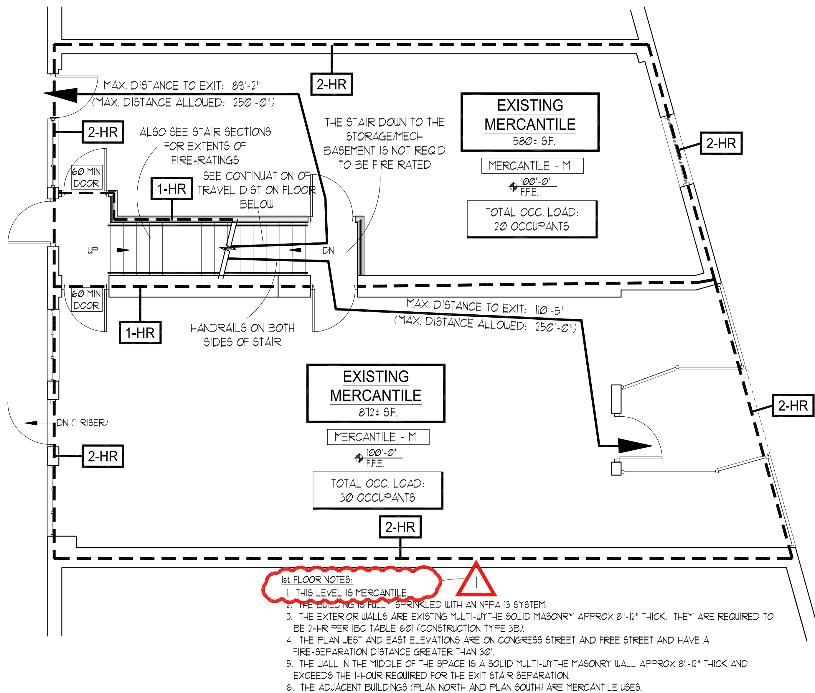
1 1st FLOOR EGRESS PLAN - 582 & 584 SCALE: 1/4" = 1'-0"
