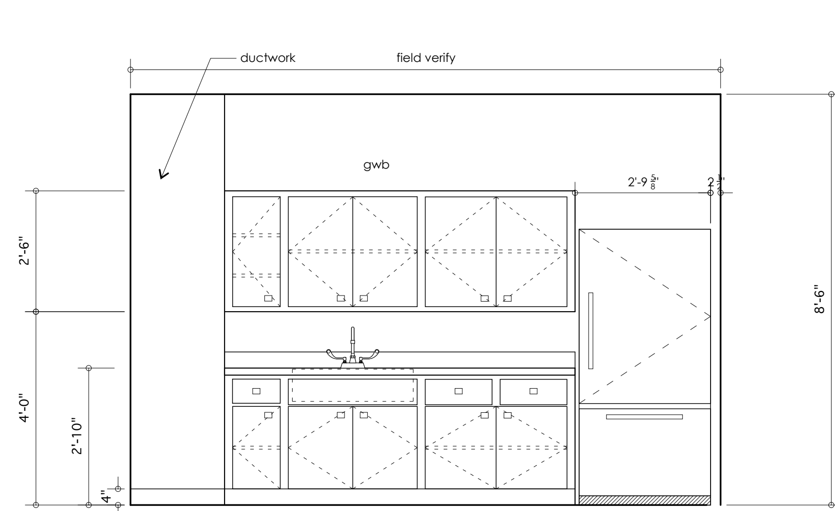
1 THIRD LEVEL BREAK ROOM ELEVATION south
