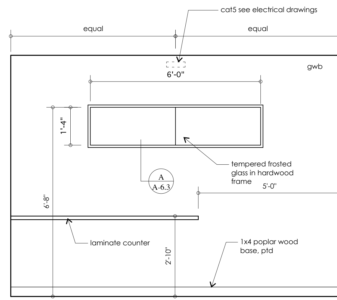
2 THIRD LEVEL BREAK ROOM ELEVATION north
