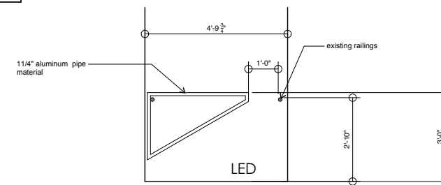
ELEVATION OF BARRIER GATE AS PER NFPA 7.7.3.2
