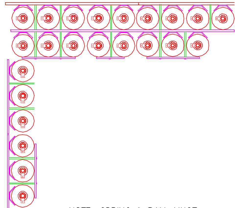
TYPICAL CYLINDER MOUNTING DETAIL SHOWING POSSIBLE CYLINDER ARRANGEMENT
