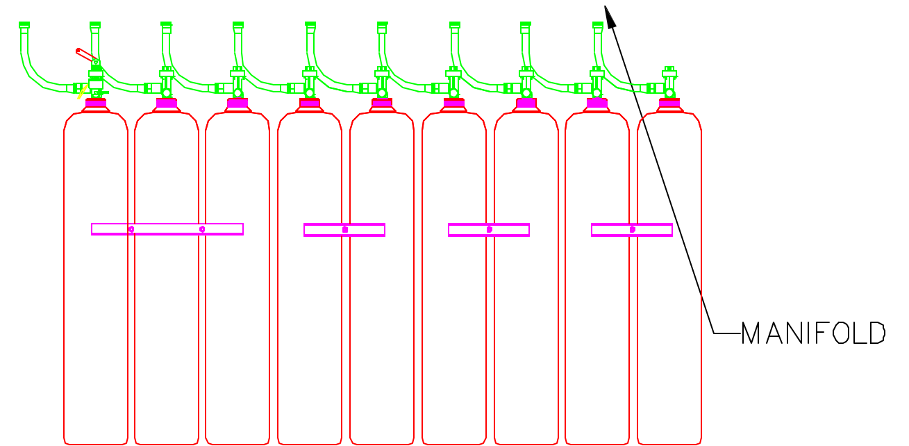
TYPICAL CYLINDER MOUNTING DETAIL SHOWING POSSIBLE CYLINDER ARRANGEMENT
