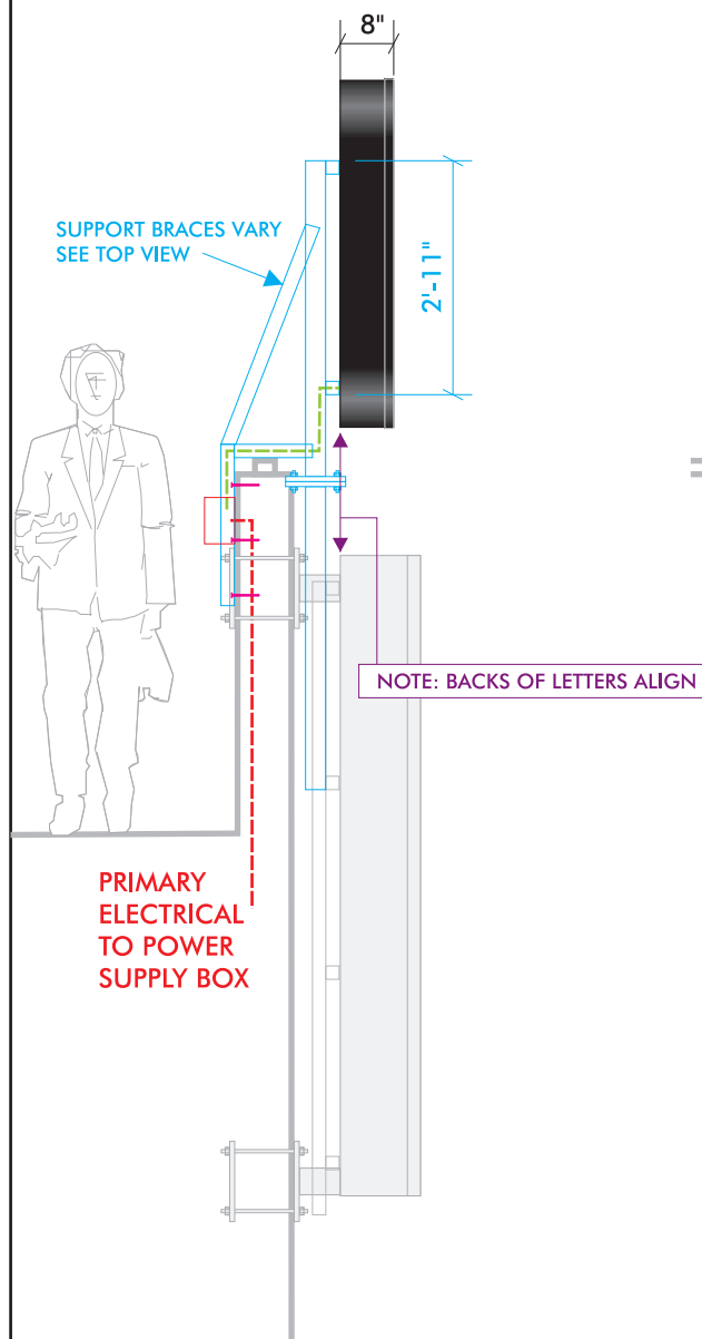
END VIEW
