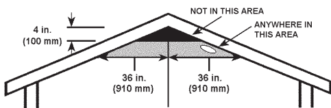
FIGURE 7: RECOMMENDED SMOKE/CO ALARM LOCATION IN ROOMS WITH SLOPED, GABLED, OR PEAKED CEILINGS.
