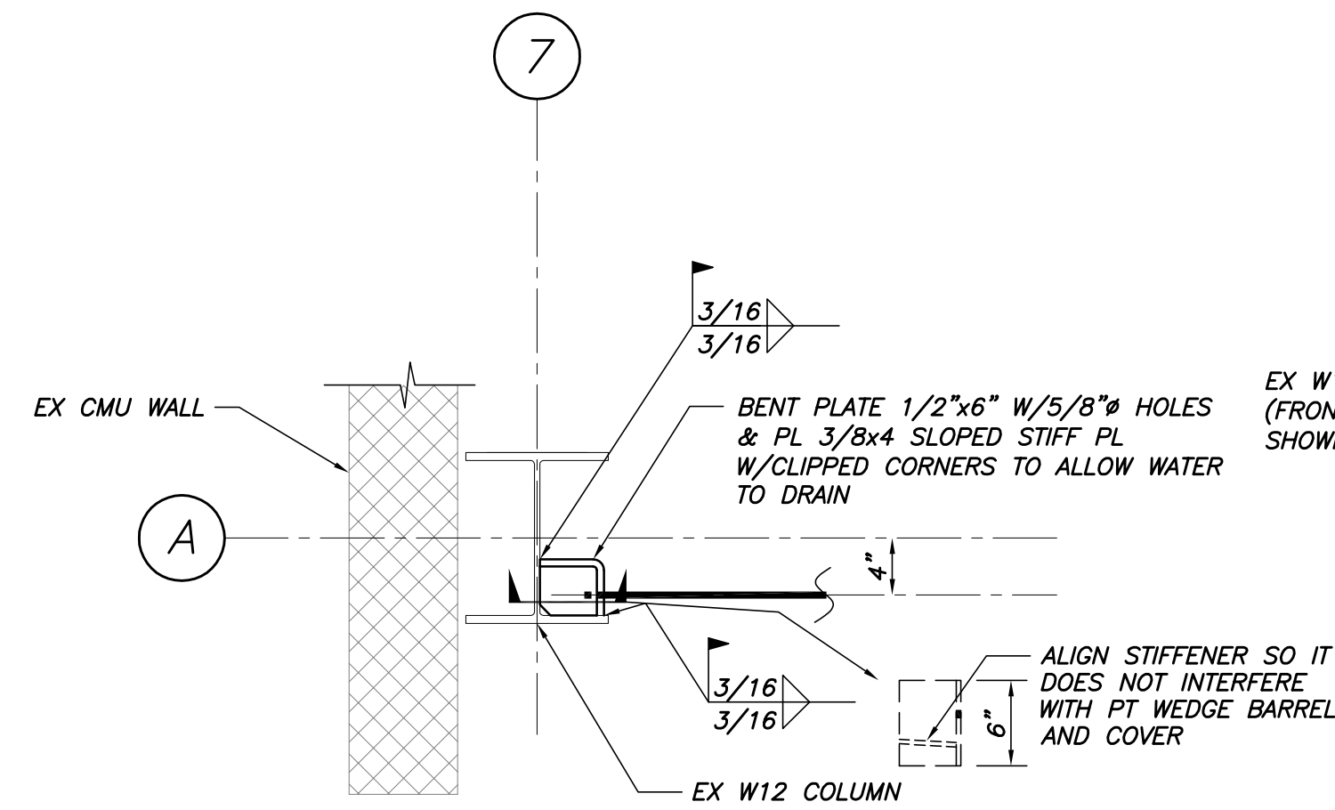
SECTION 7 1"=1'-0"
