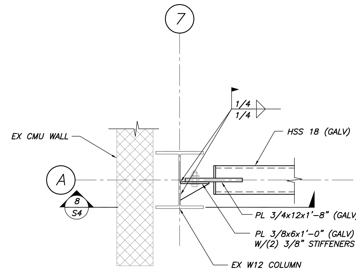
SECTION 6 1"=1'-0"
