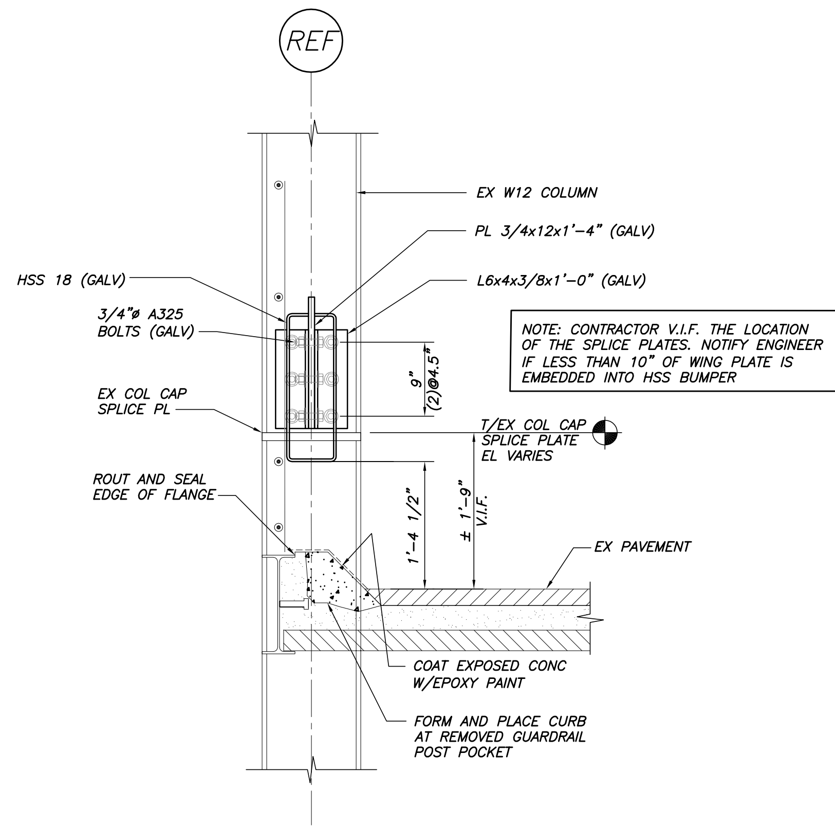
SECTION 1 1"=1'-0"
