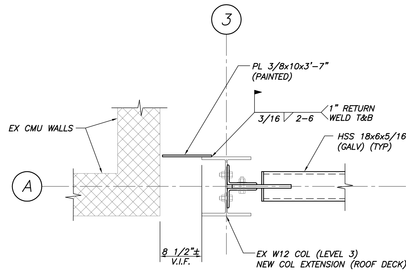
SECTION 5 1"=1'-0"
