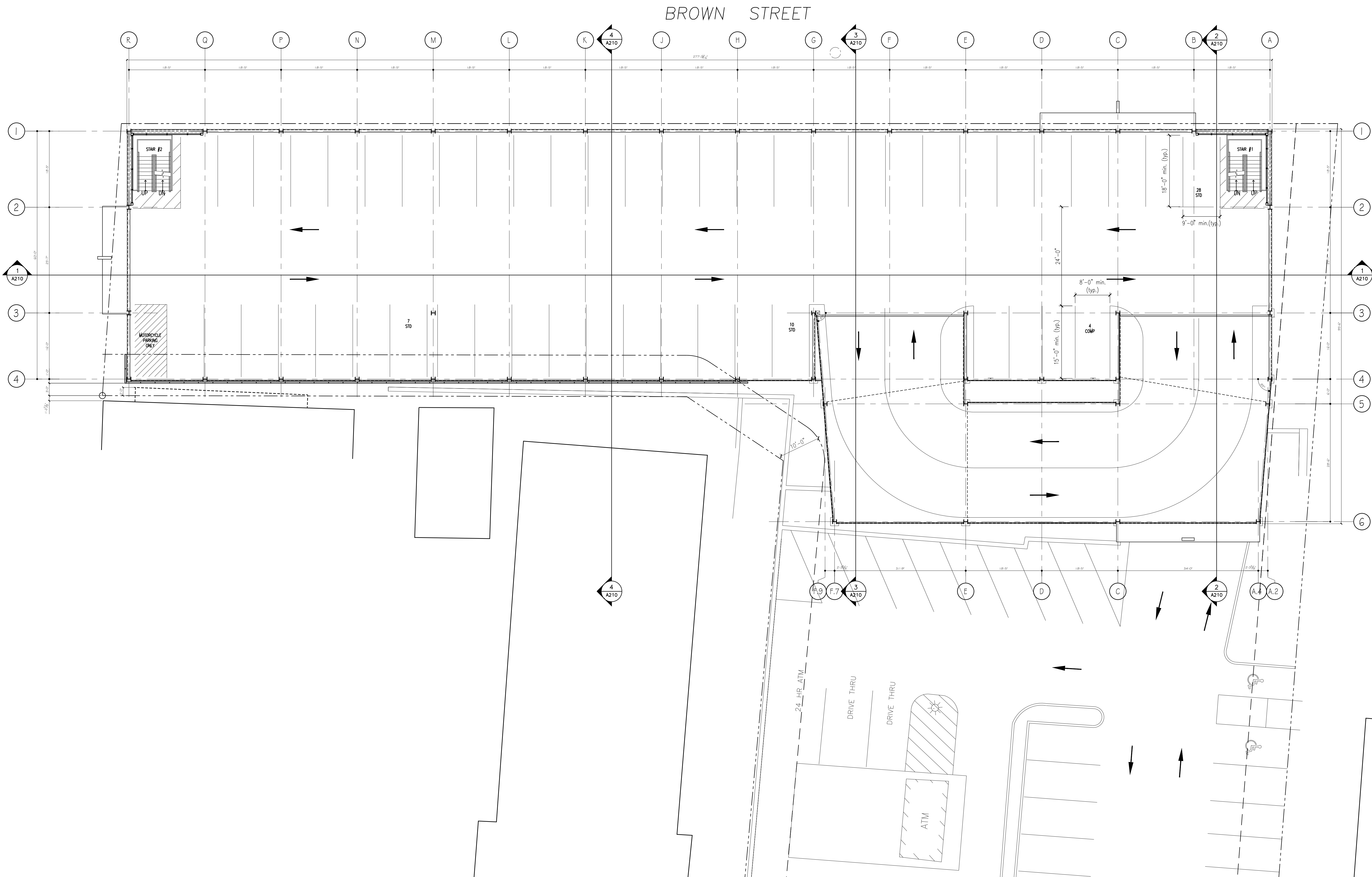
1 THIRD LEVEL FLOOR PLAN ~ SCALE: 3/32" = 1'-0"
