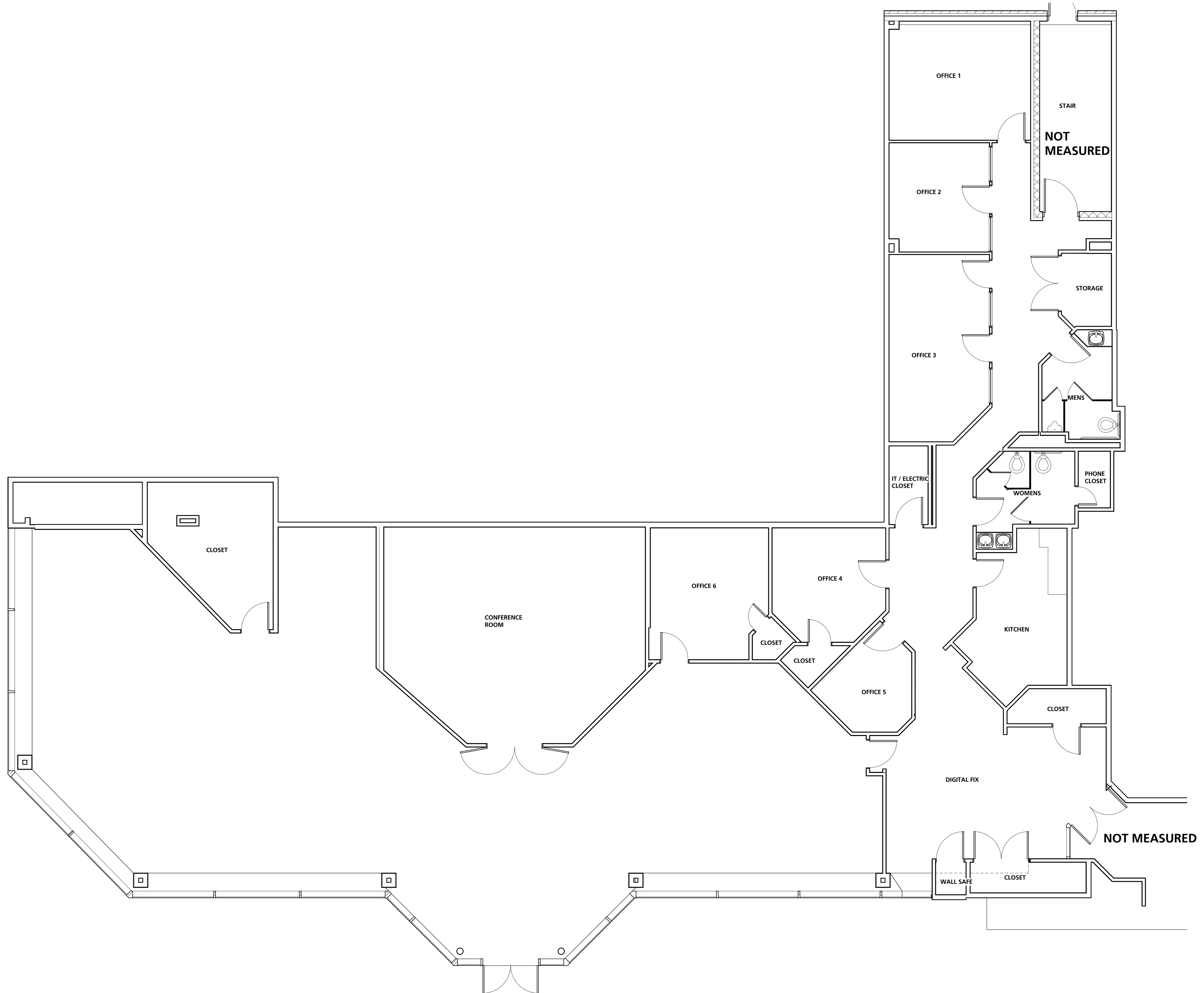
1 EXISTING FIRST FLOOR PLAN AX100 3/16" = 1'-0"
