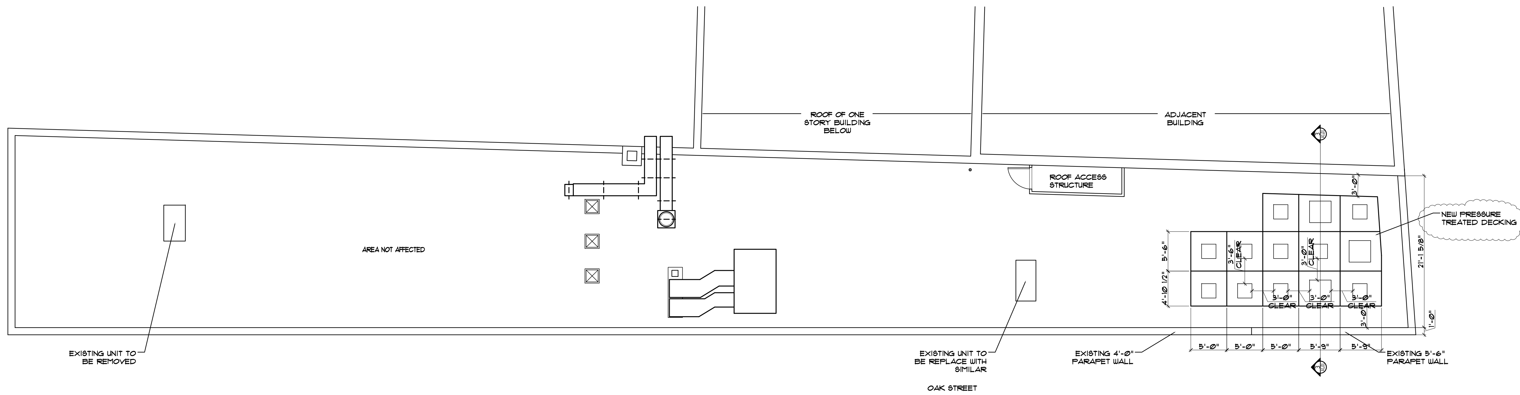
1 | PROPOSED ROOF DECK PLAN SCALE: 1/8"=1'-0"
