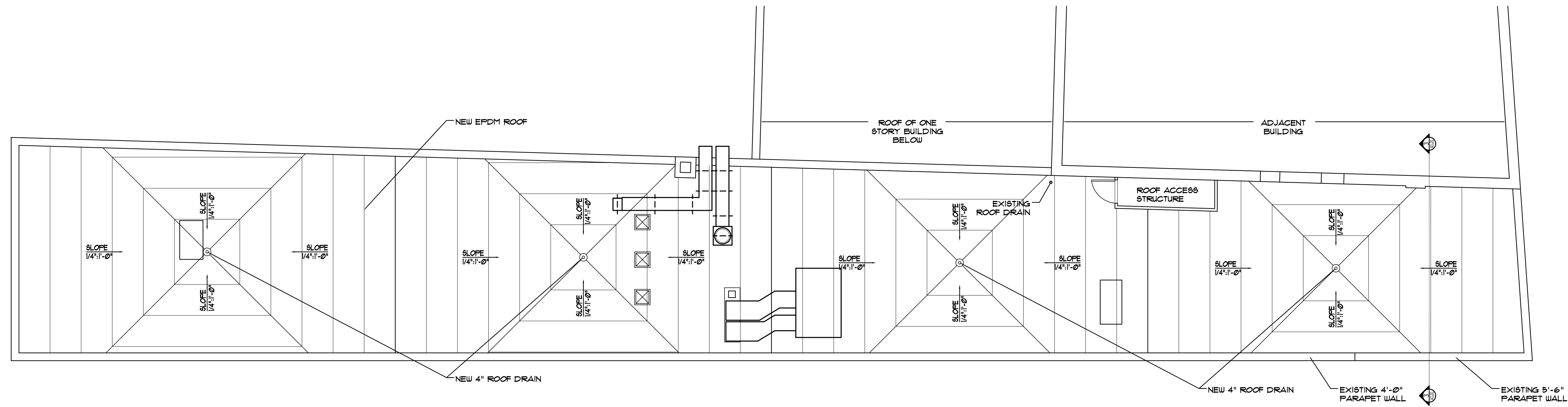
2 | PROPOSED ROOF DRAINAGE PLAN SCALE: 1/8"=1'-0"
