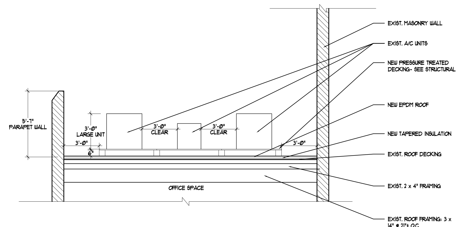
3 | ROOF SECTION SCALE: 1/4"=1'-0"
