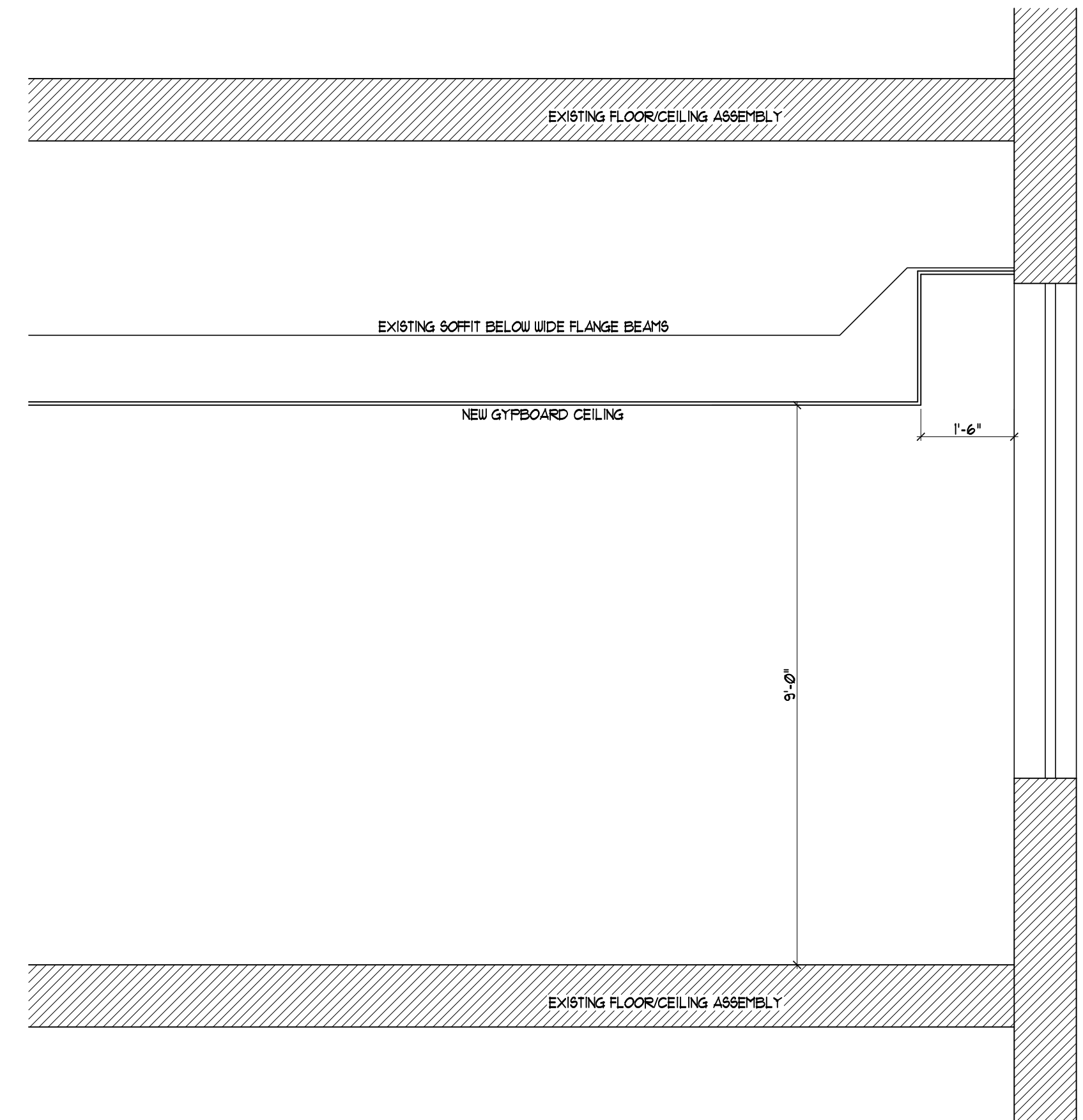
2 TYPICAL SECTION AT WINDOW SCALE: 1/2" = 1'-0"
