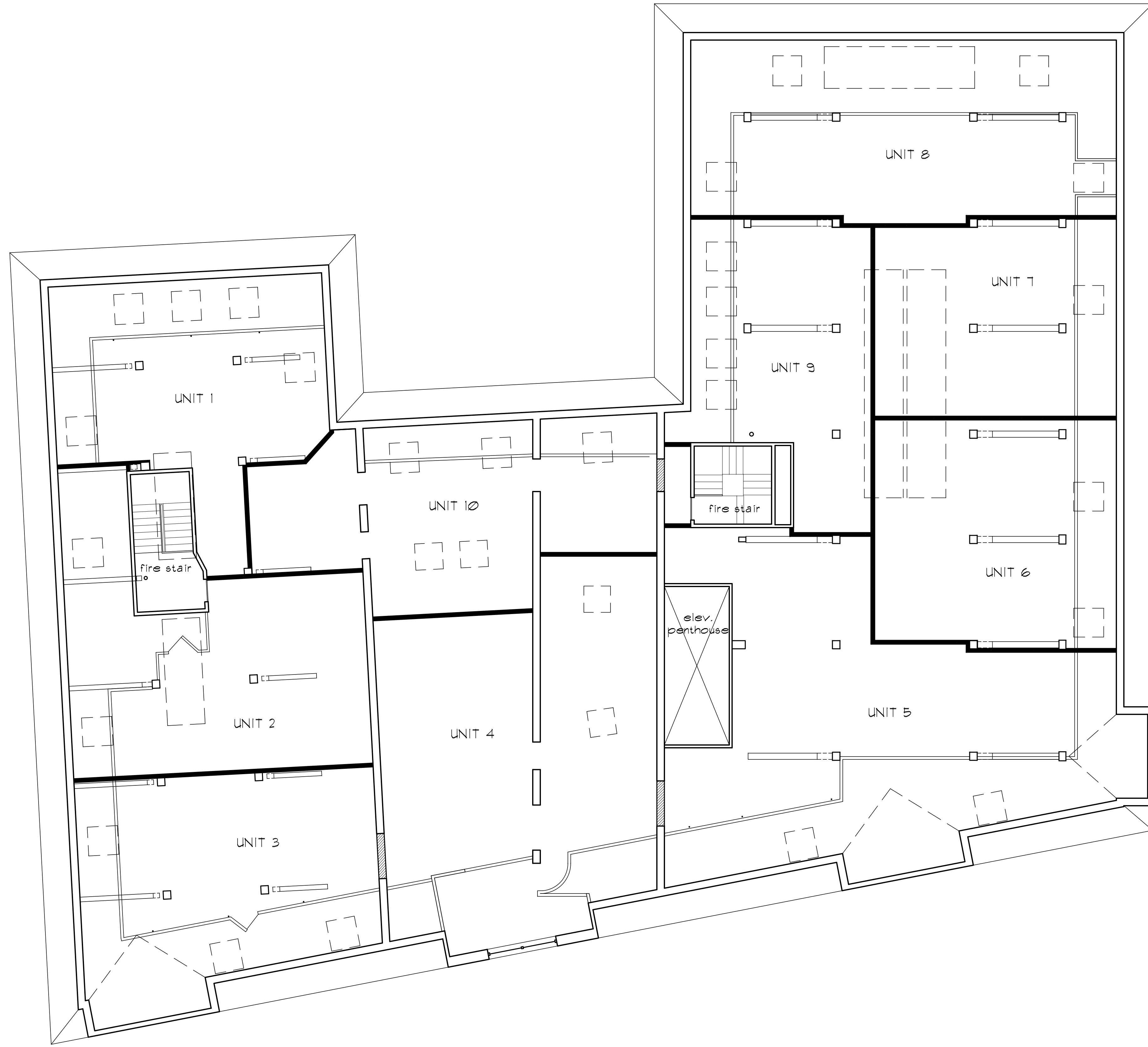
① SIXTH FLOOR PLAN SCALE : 1/8" = 1'-0"
