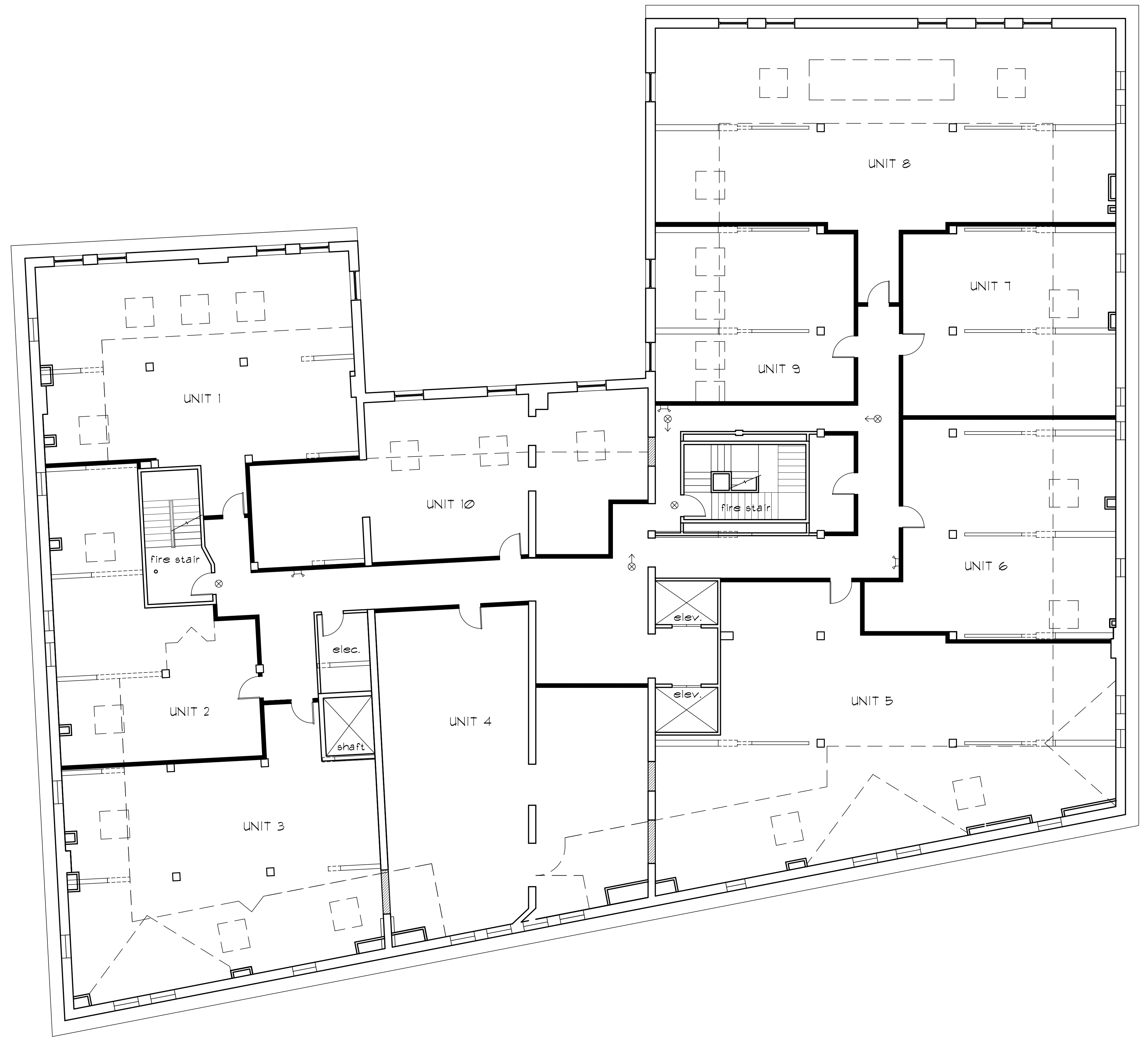
① FIFTH FLOOR PLAN SCALE : 1/8" = 1'-0"
