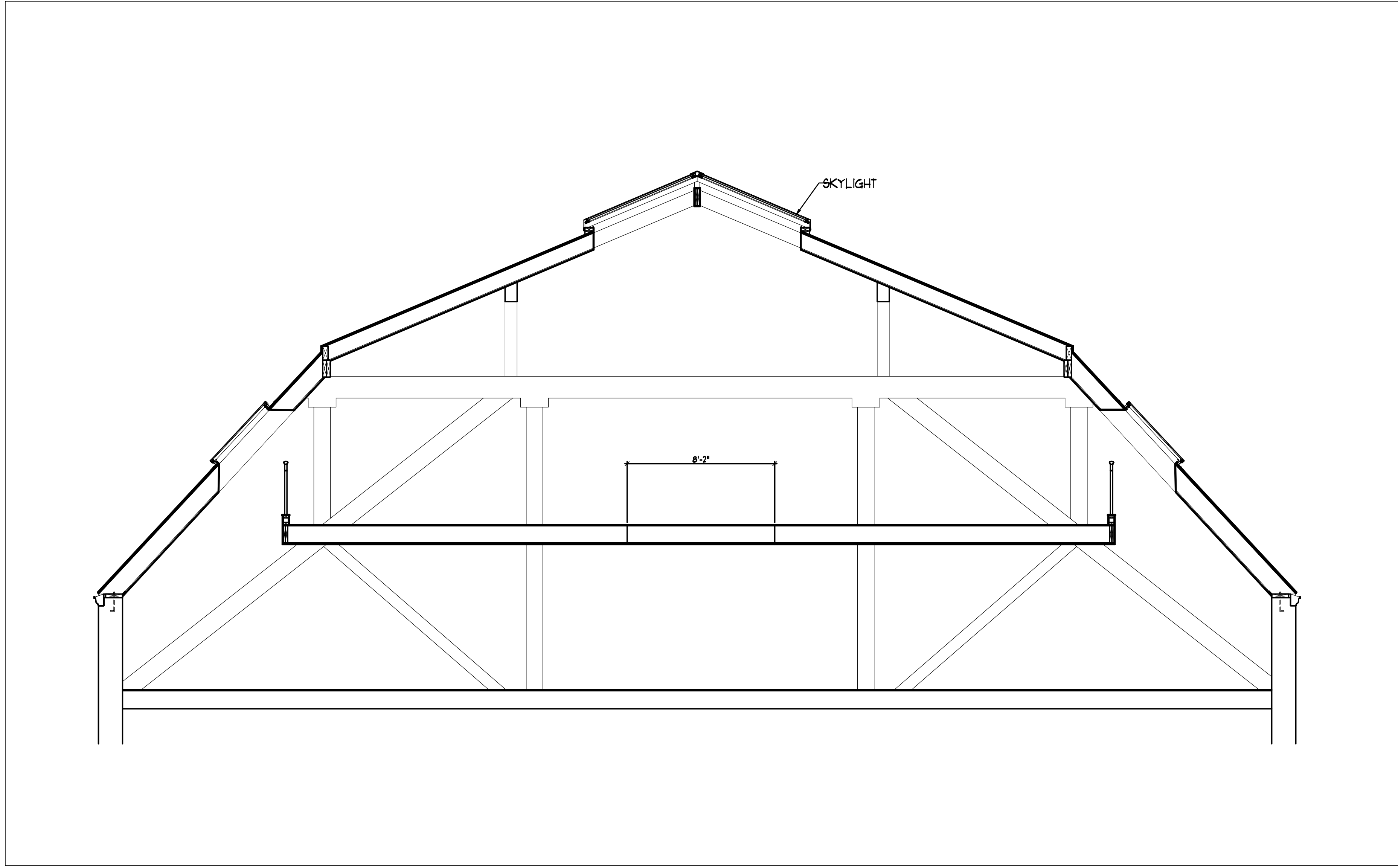
1 BUILDING SECTION - UNIT 7 SCALE : 1/4" = 1'-0"
