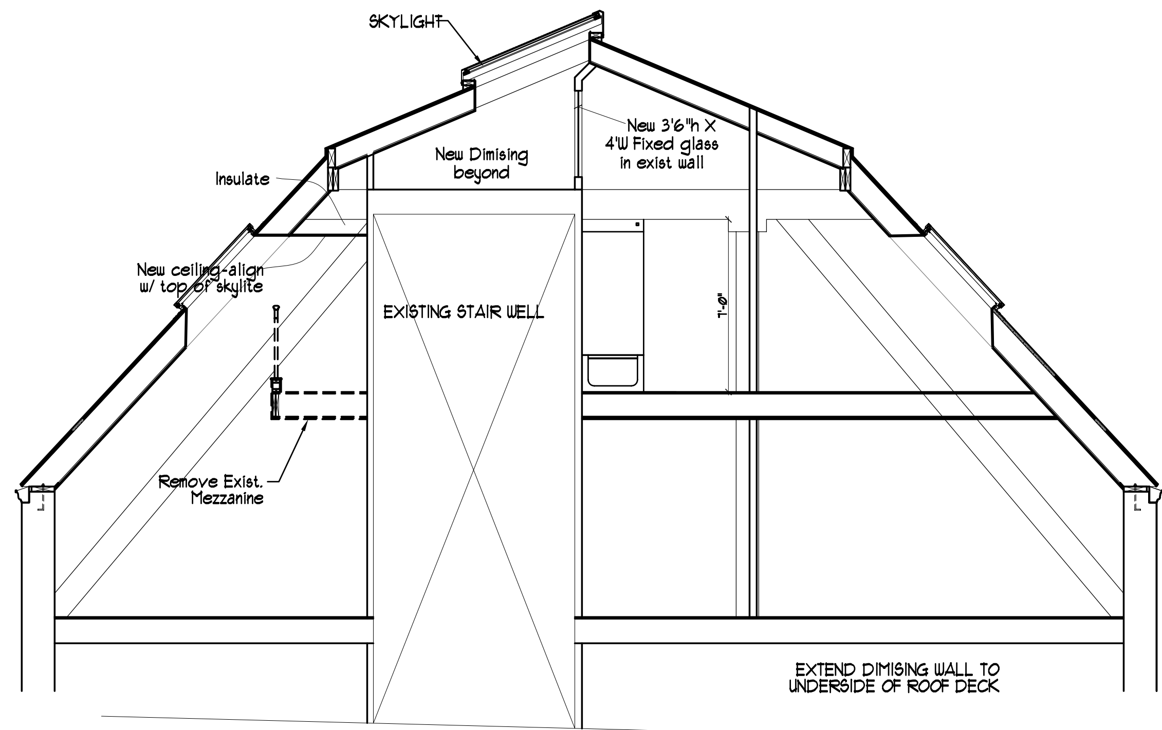
① SECTION - UNIT 2 SCALE : 1/4" = 1'-0"
