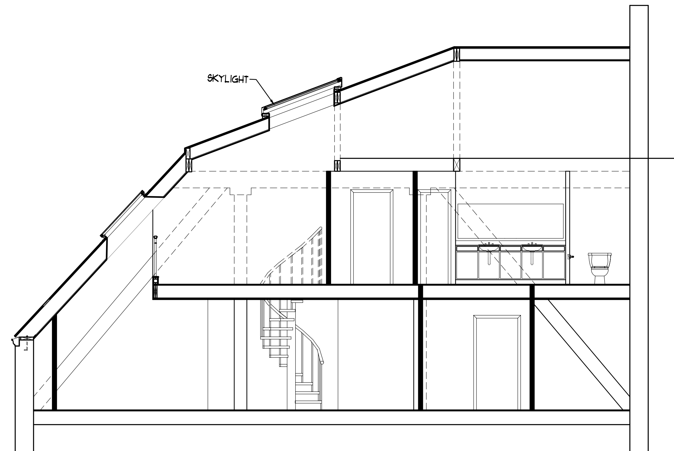
② SECTION - UNIT 2 SCALE : 1/4" = 1'-0"
