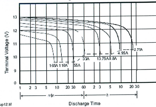
UB12550/SA12550 discharge characteristics (25°C/77°F)
