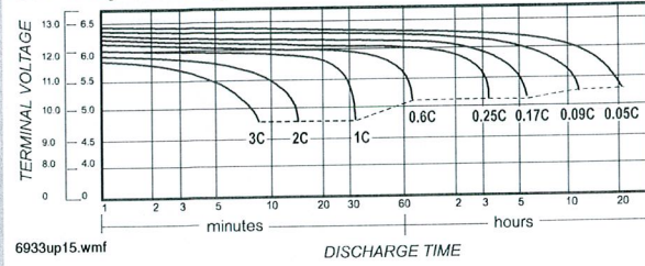
Summary discharge current vs. time curve (25°C/77°F)
