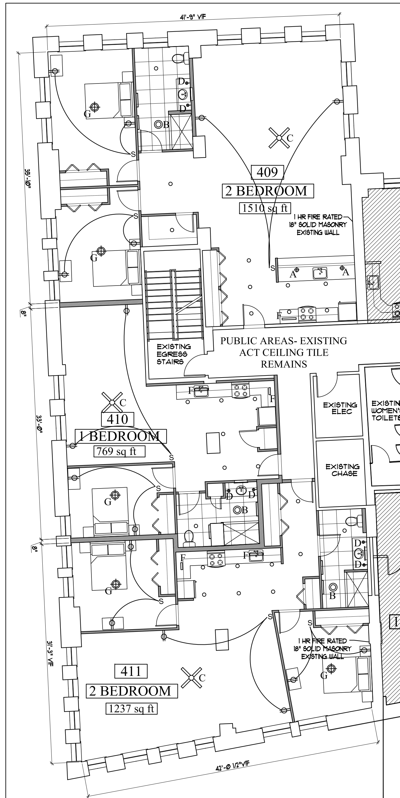
FOURTH FLOOR REFLECTED CEILING PLAN SCALE: 1/8" = 1'-0"
