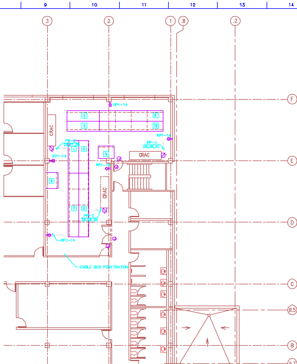
E9 SECOND FLOOR POWER PART PLAN FILENAME: 1/8"=1'-0"
