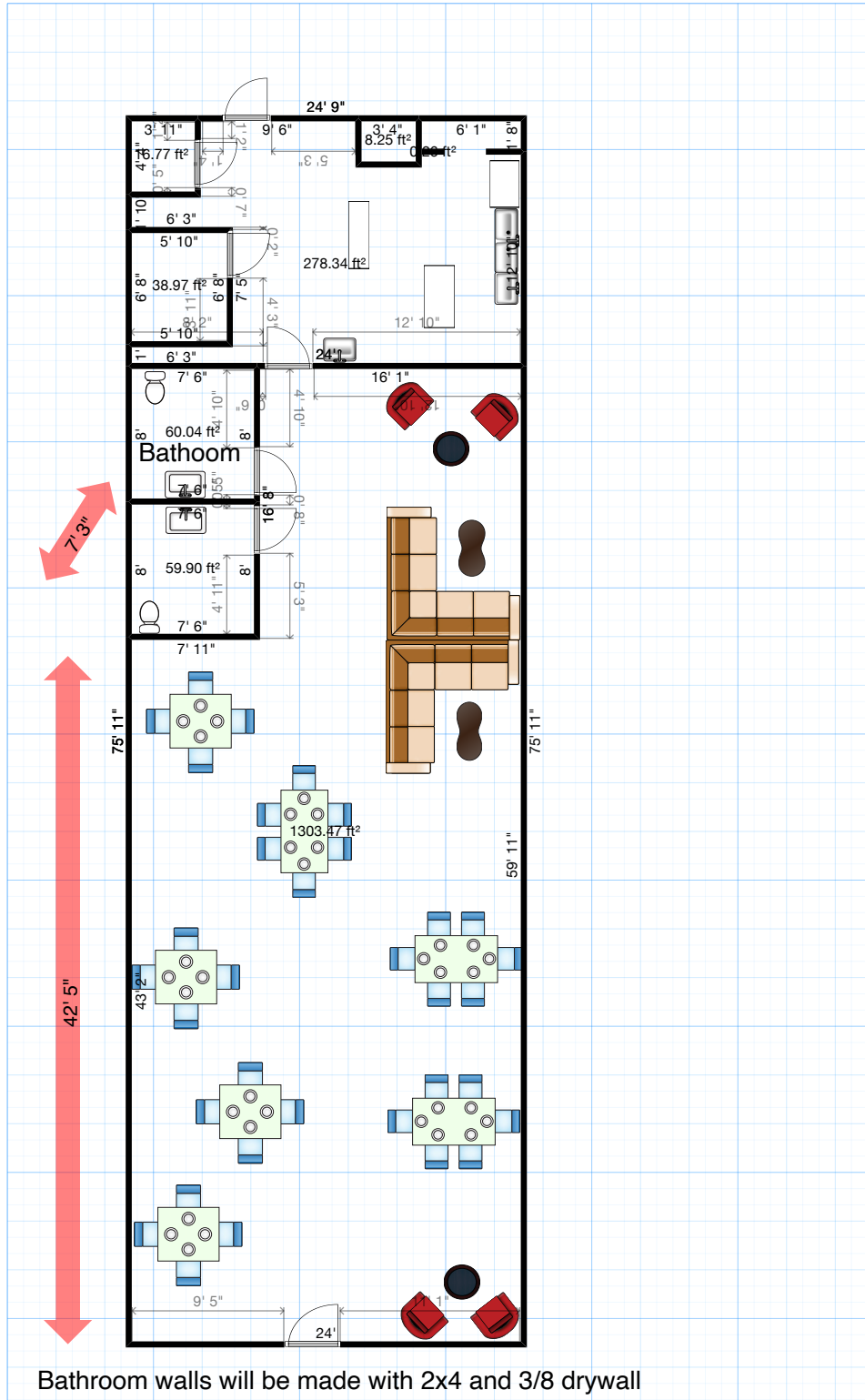
Floor 1
