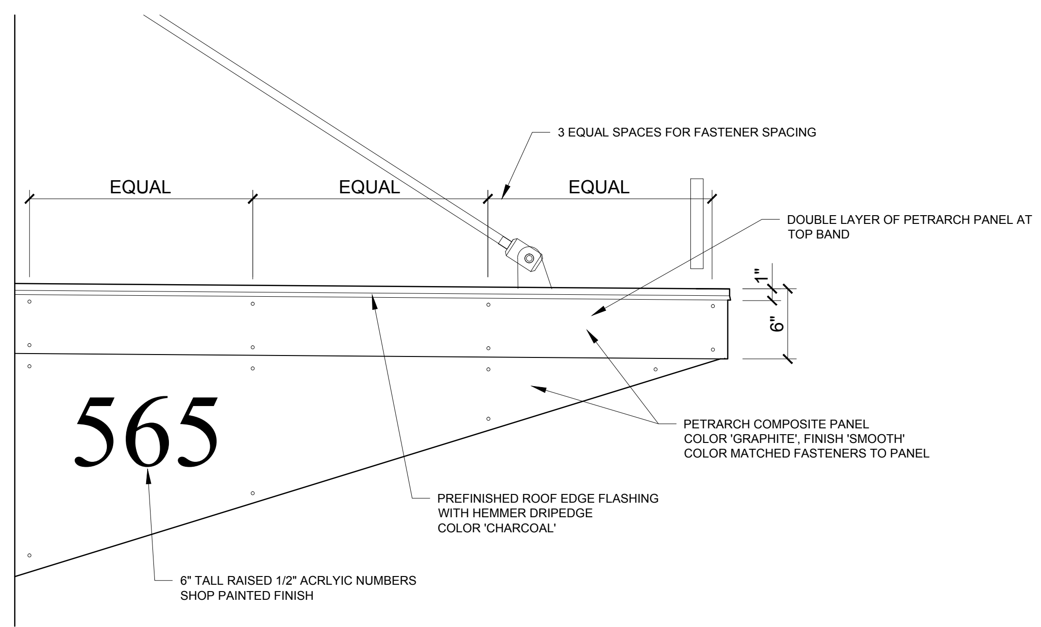
2 CANOPY SIDE ELEVATION DETAIL (OTHER SIDE SIMILAR) 1:12" = 1'-0"
