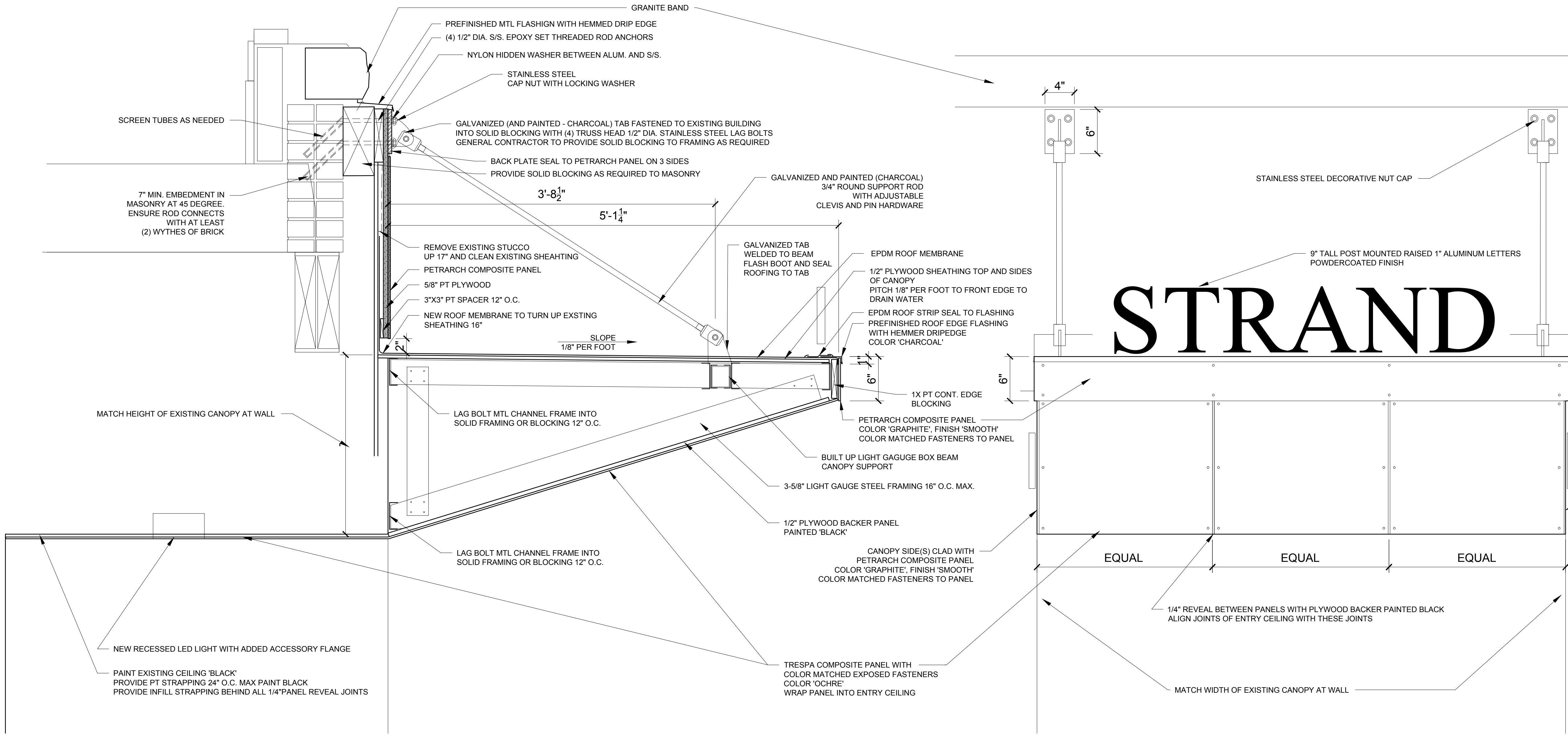
2 SECTION DETAIL 1:12" = 1'-0"
