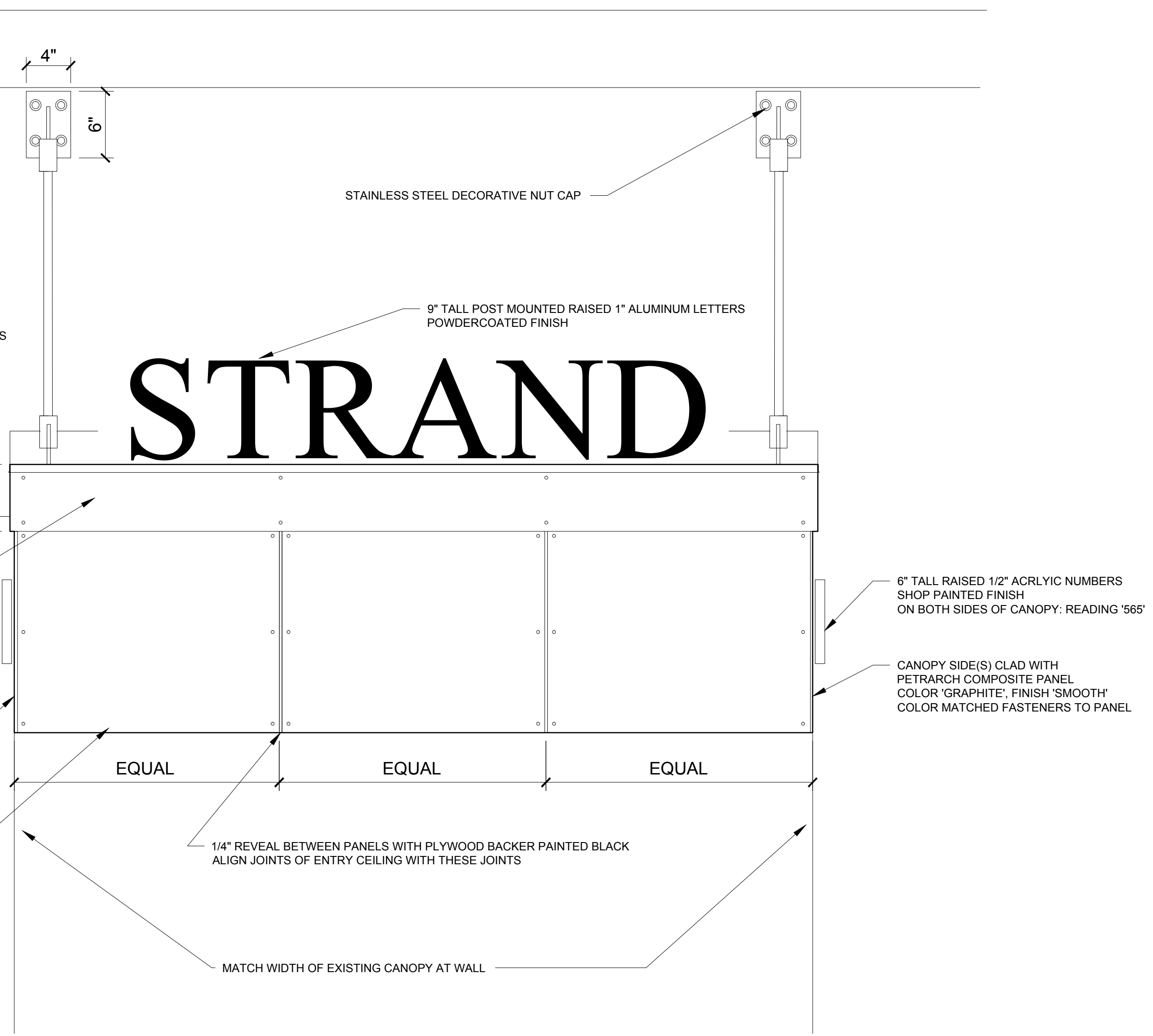
1 ELEVATION DETAIL 1:12" = 1'-0"
