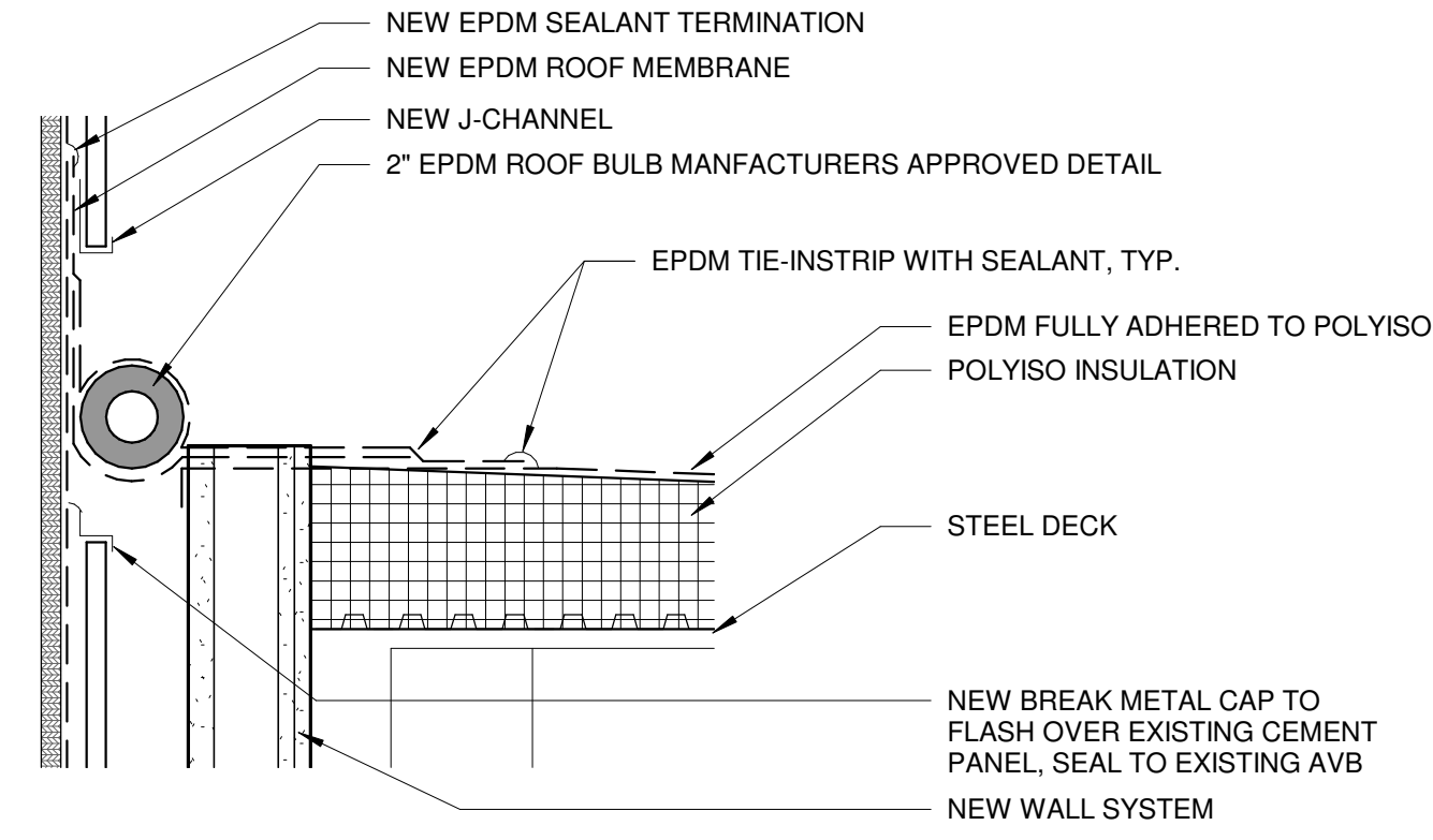
2 BUILDING CONNECTION DETAIL 1 1/2" = 1'-0"
