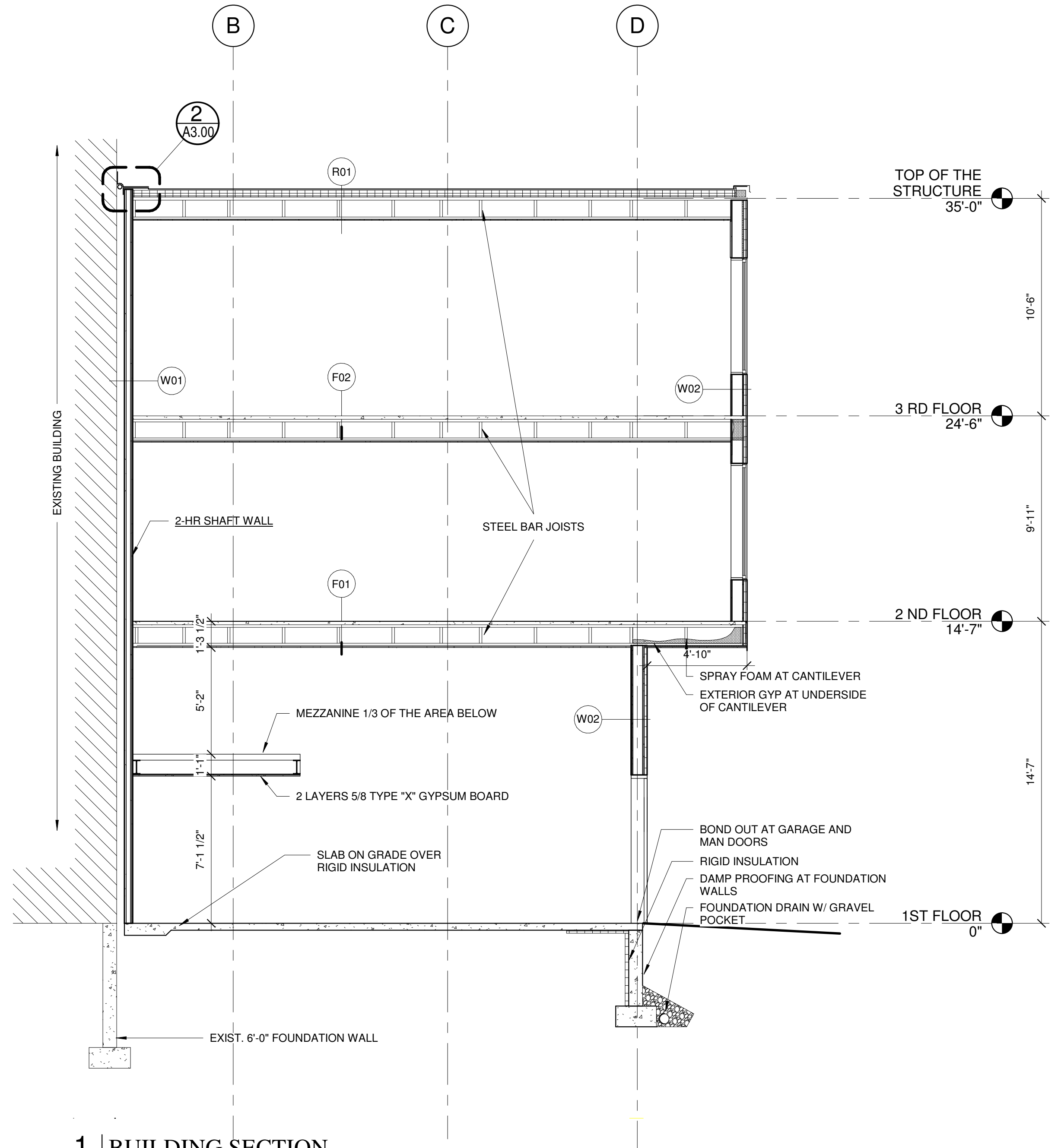
1 BUILDING SECTION 1/4" = 1'-0"
