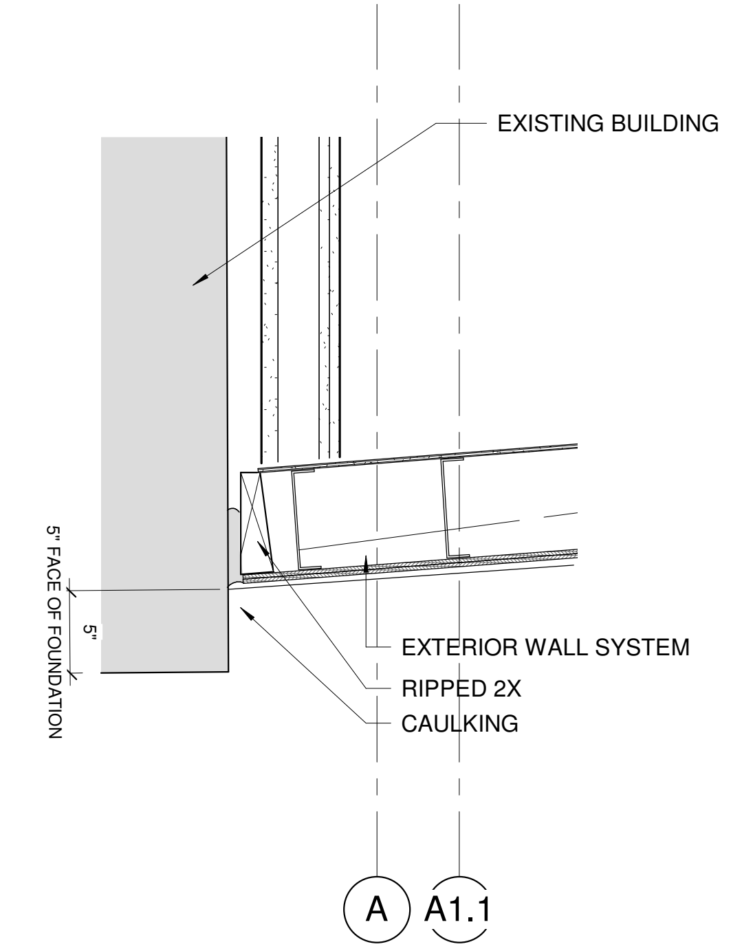
3 1ST FLOOR DETAIL 1 1/2" = 1'-0"
