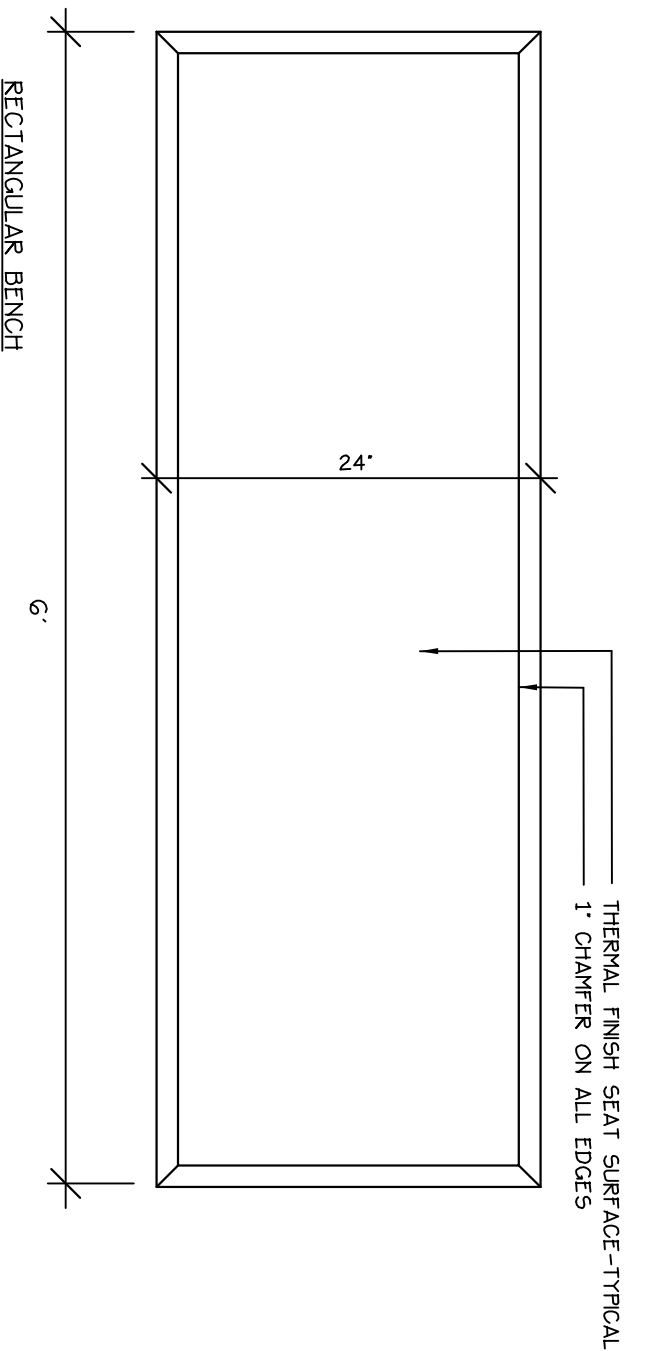
2 PLAN VIEW - 6' GRANITE BENCH NOT TO SCALE
