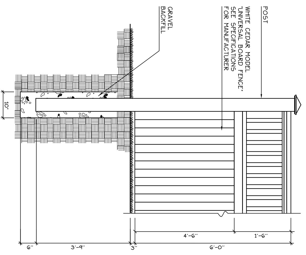
3 SOLID WOOD FENCE NOT TO SCALE
