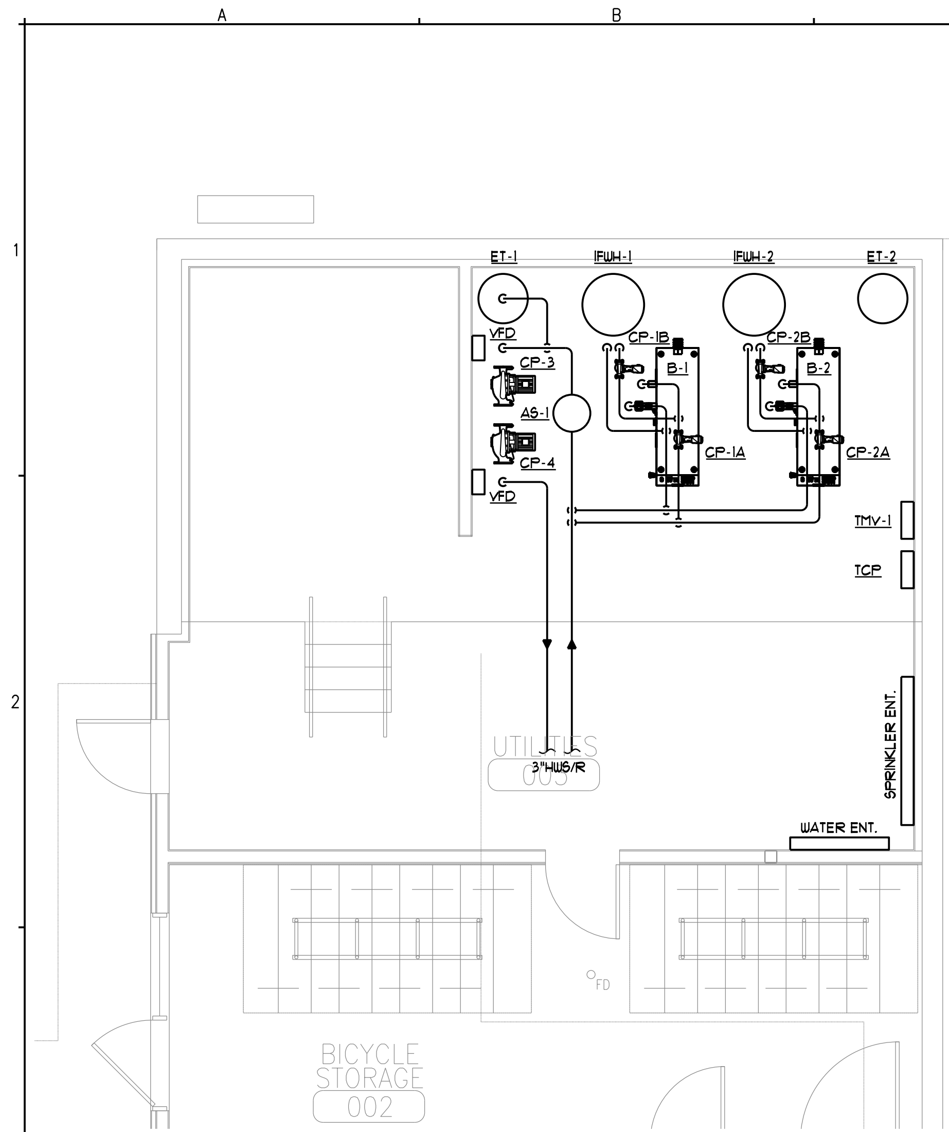
MECHANICAL ROOM ENLARGED PLAN SCALE - 1/4" = 1'-0"
