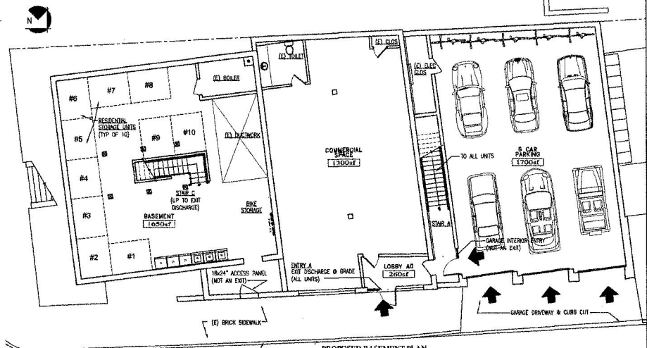
PROPOSED BASEMENT PLAN SCALE: 1/8" = 1'-0"
