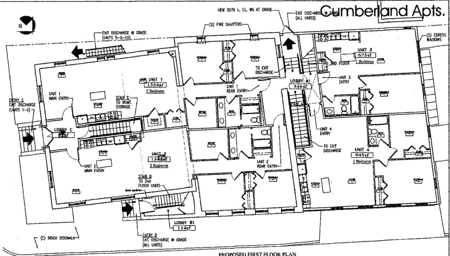
PROPOSED FIRST FLOOR PLAN SCALE: 1/8" = 1'-0"
