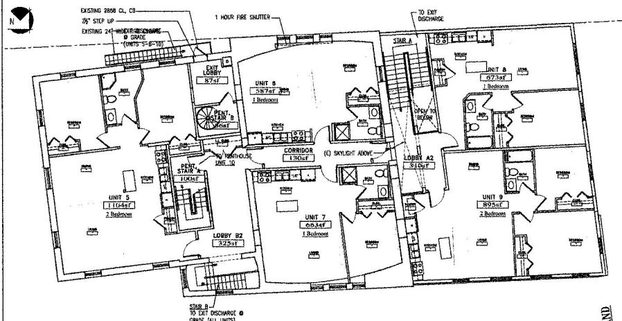
PROPOSED SECOND FLOOR PLAN SCALE: 1/8" = 1'-0"
