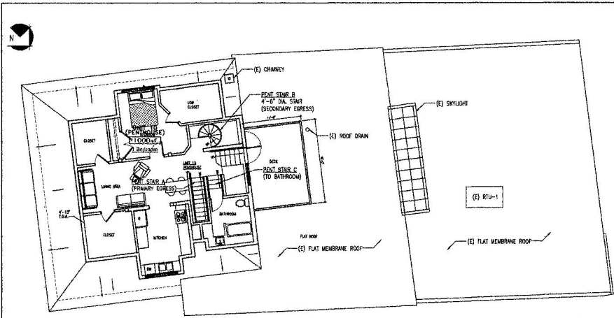
PROPOSED PENTHOUSE PLAN SCALE: 1/8" = 1'-0"
