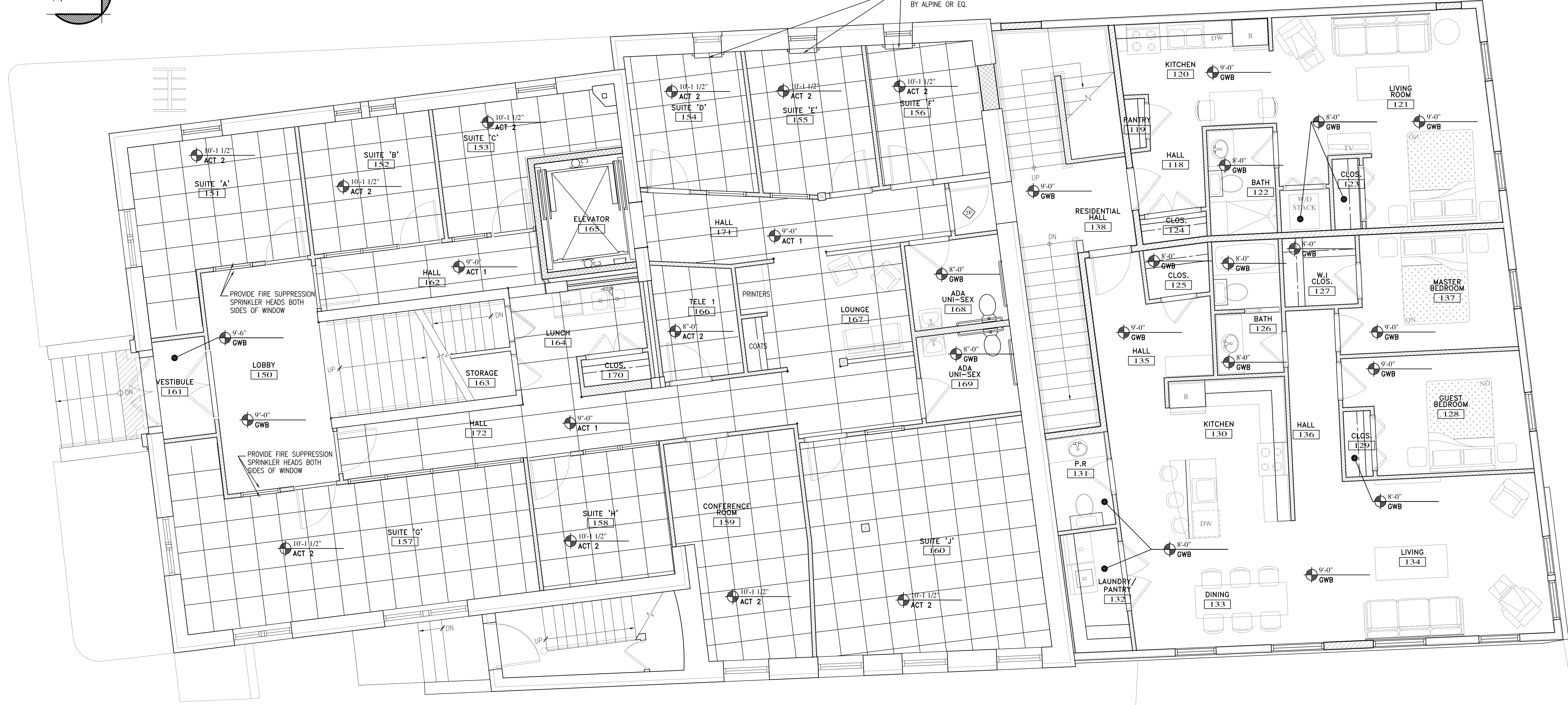
FIRST FLOOR REFLECTED CEILING PLAN SCALE: 1/4" = 1'-0"
