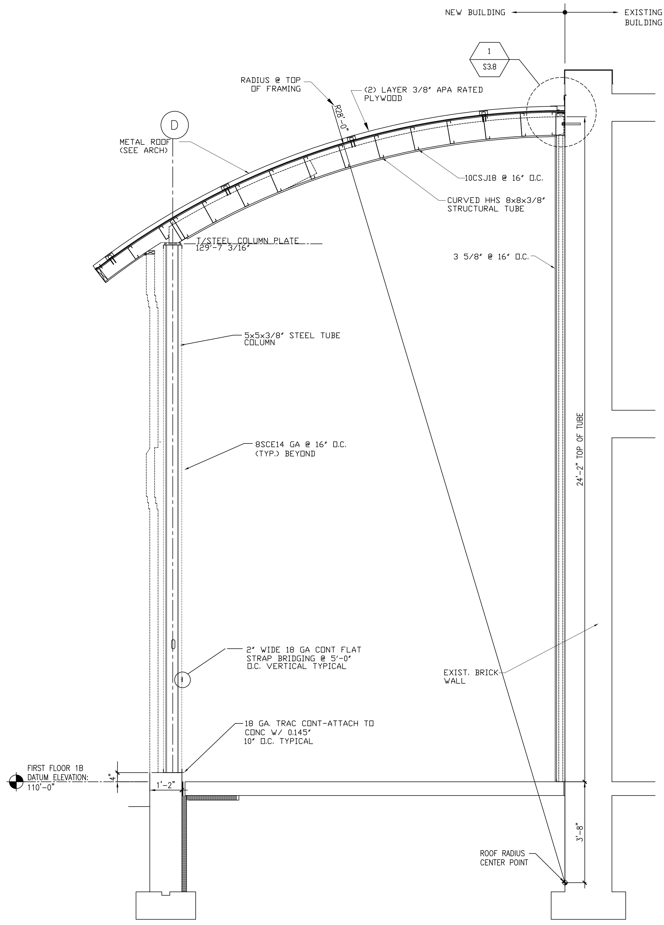
SECTION E 1/2" = 1'-0" S3.1
