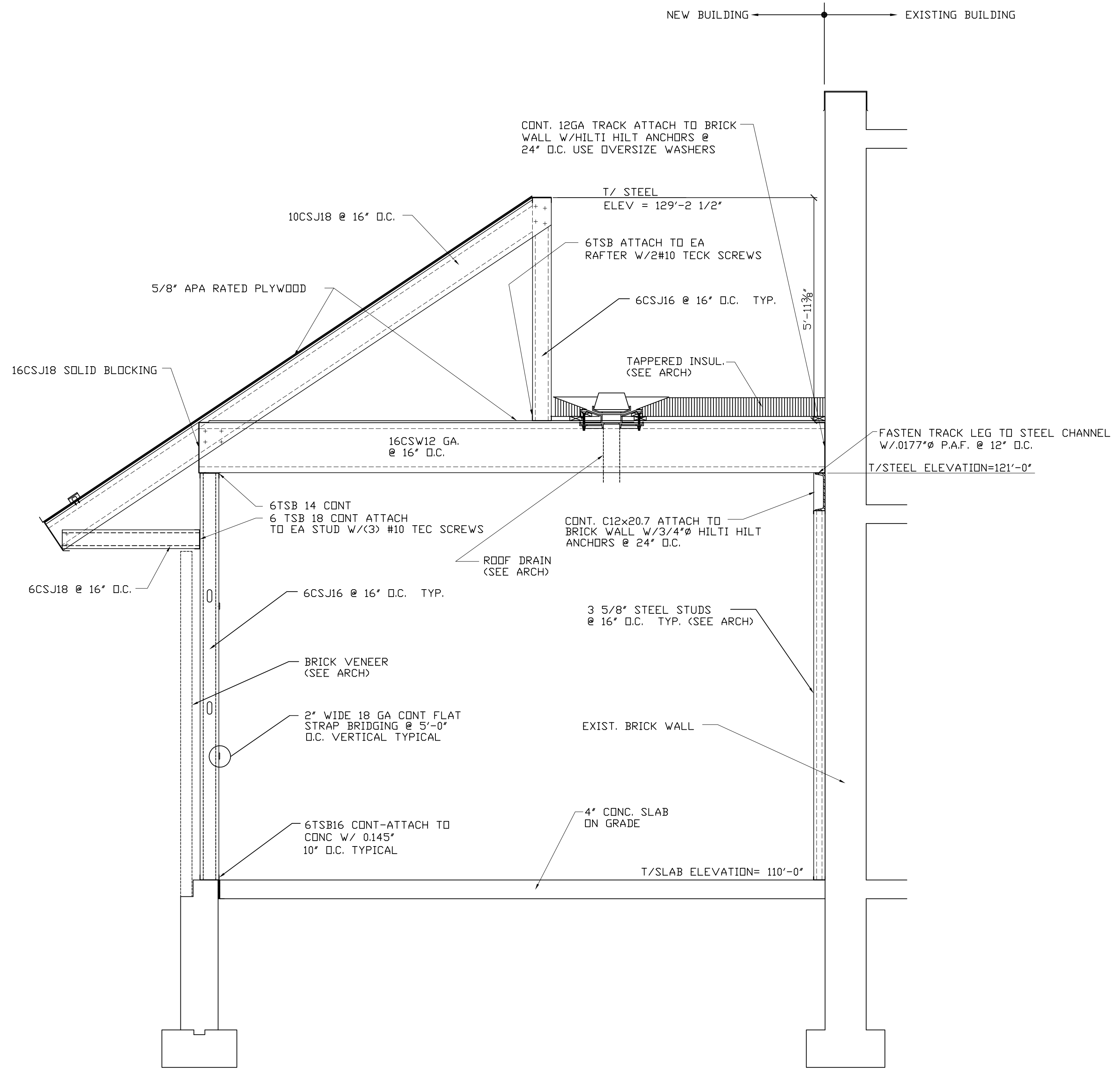
SECTION F 1/2" = 1'-0" S3.1
