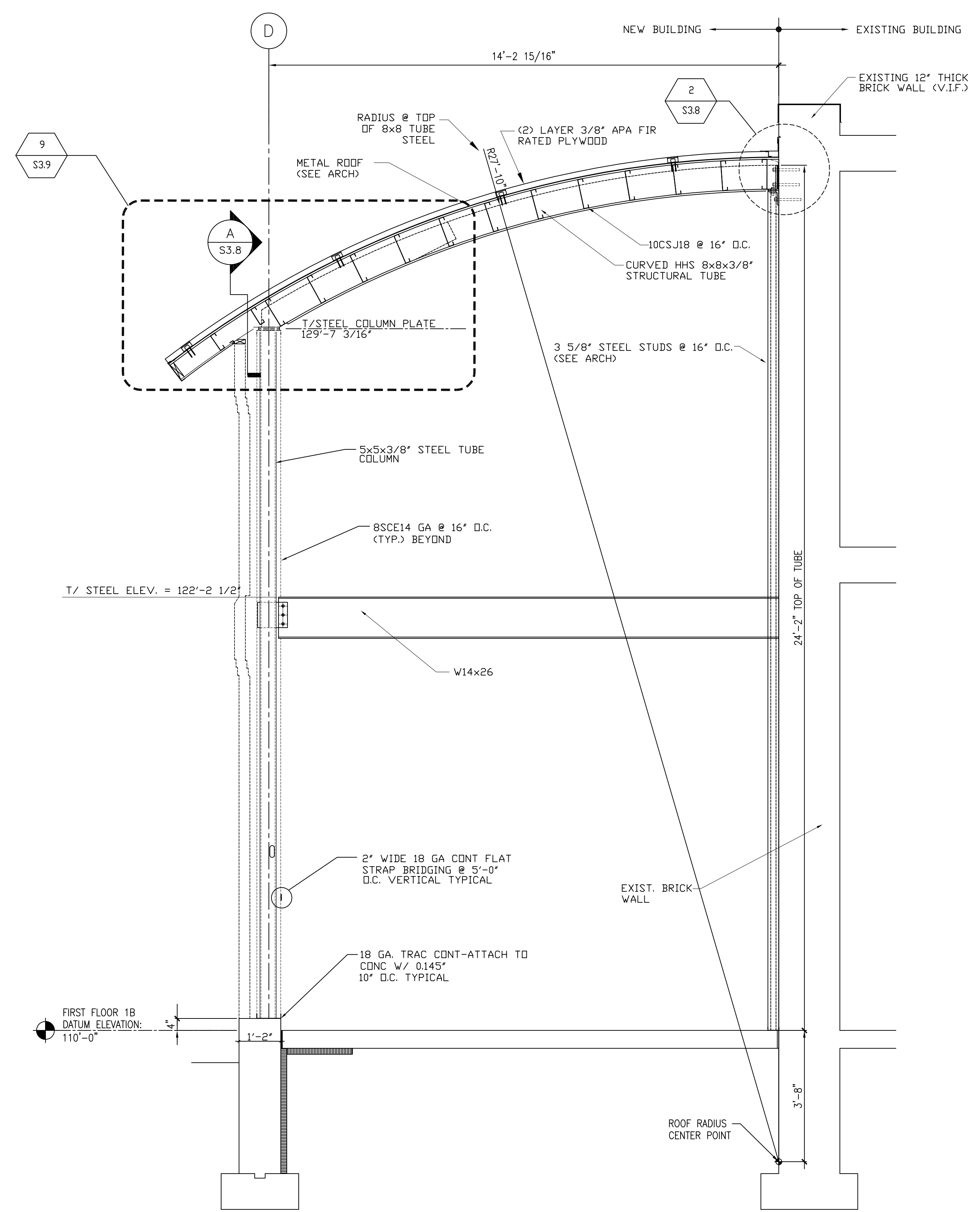
SECTION @ 5 LINE D 1/2" = 1'-0" S3.3
