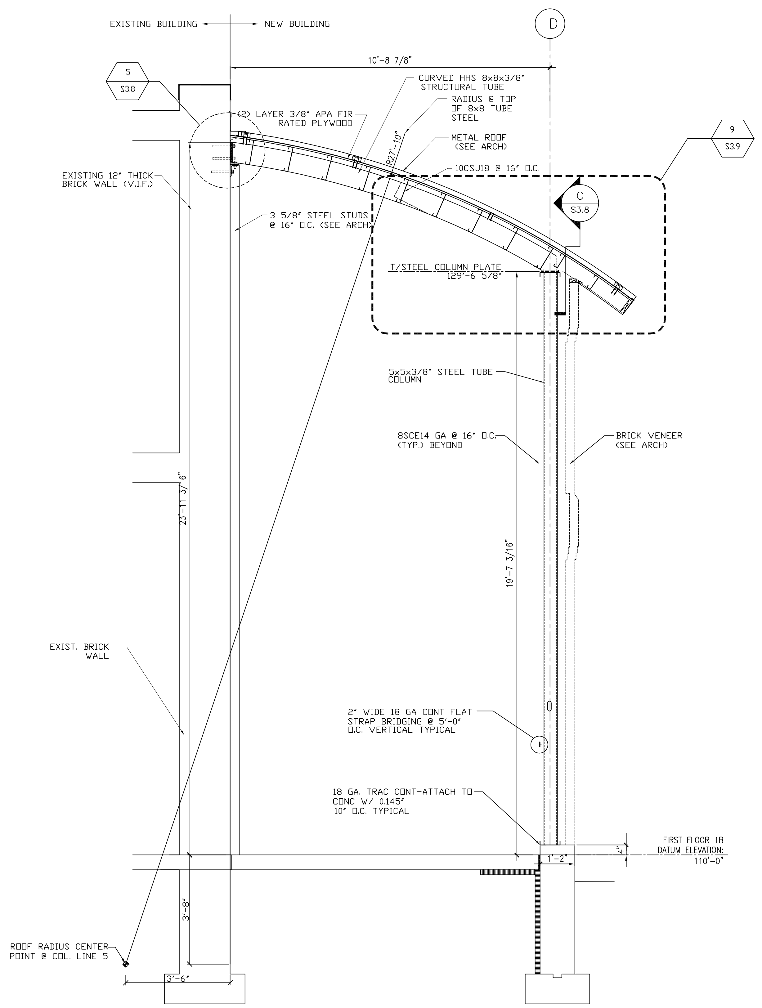
SECTION @ 8 LINE A 1/2" = 1'-0" S3.2
