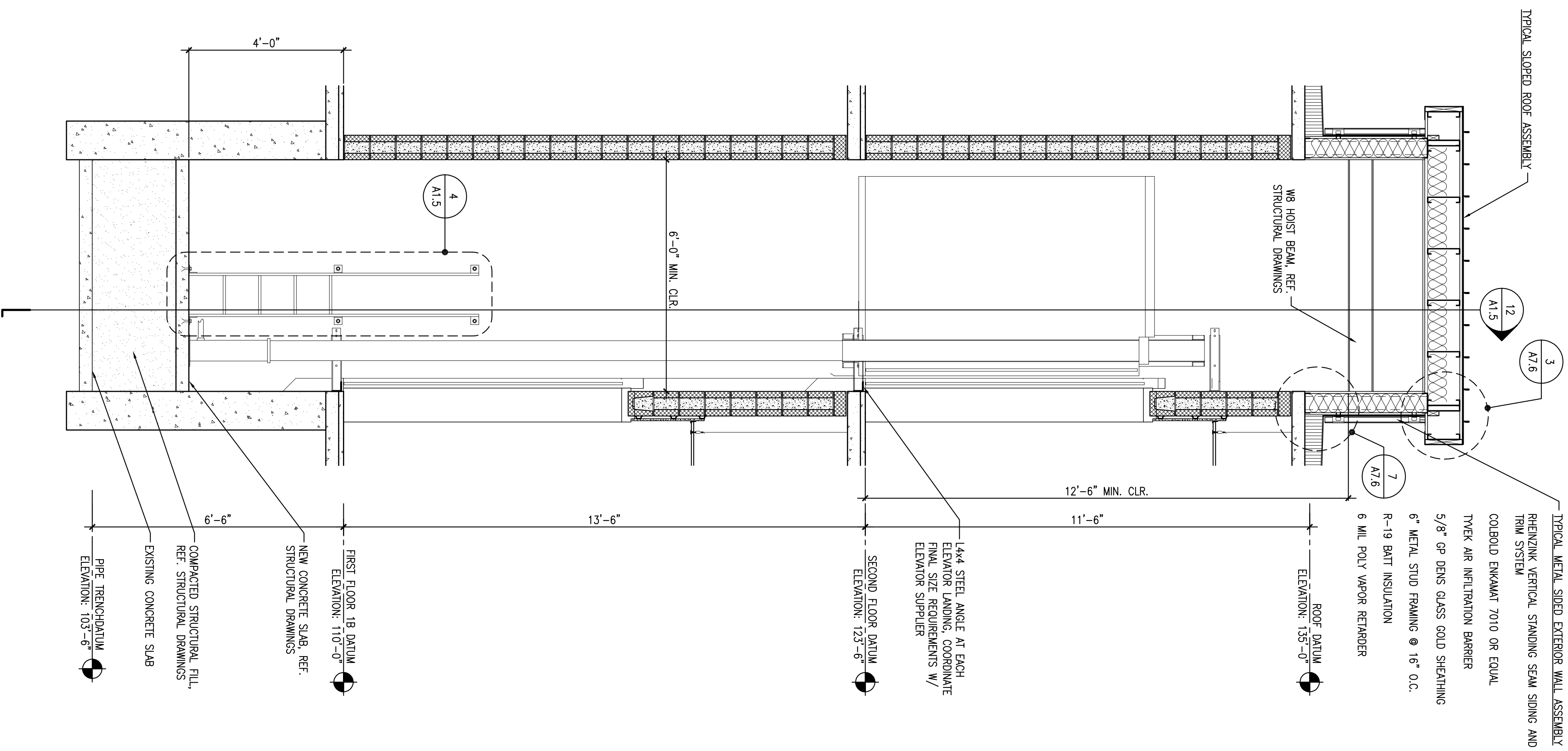
11 SECTION @ ELEVATOR REFERENCED FROM: SCALE: 1/2" = 1'-0"
