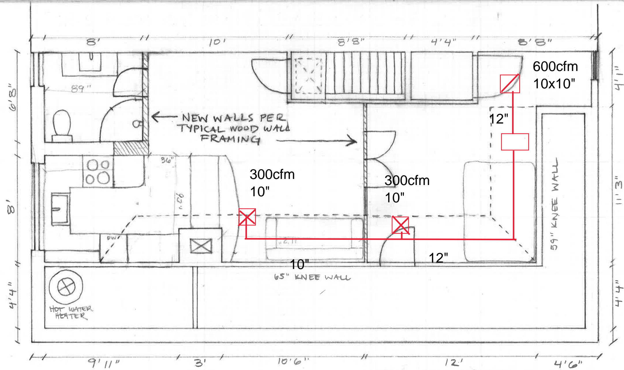
THIRD FLOOR RENOVATION PLAN @ 1" = 1/4" SCALE
