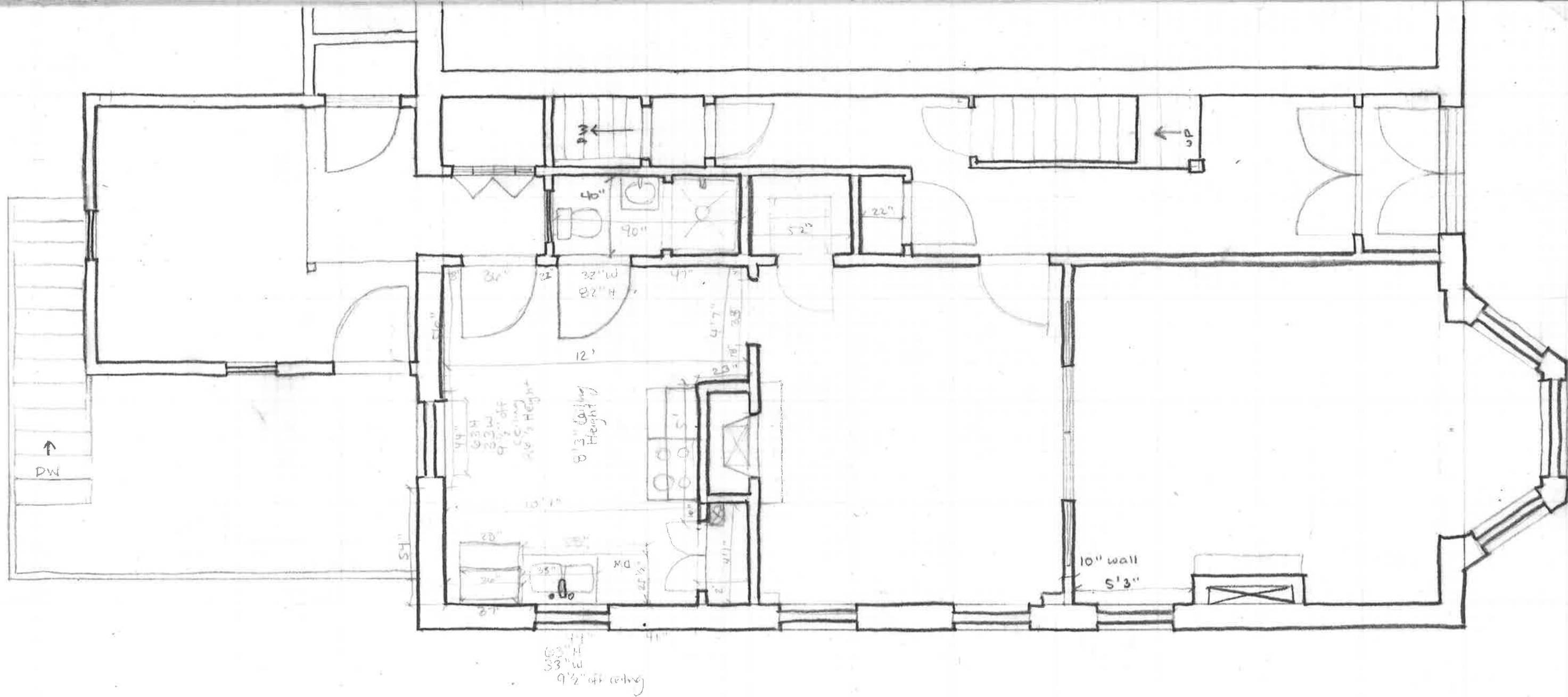
FIRST FLOOR EXISTING @ 1" = 1/4" SCALE
