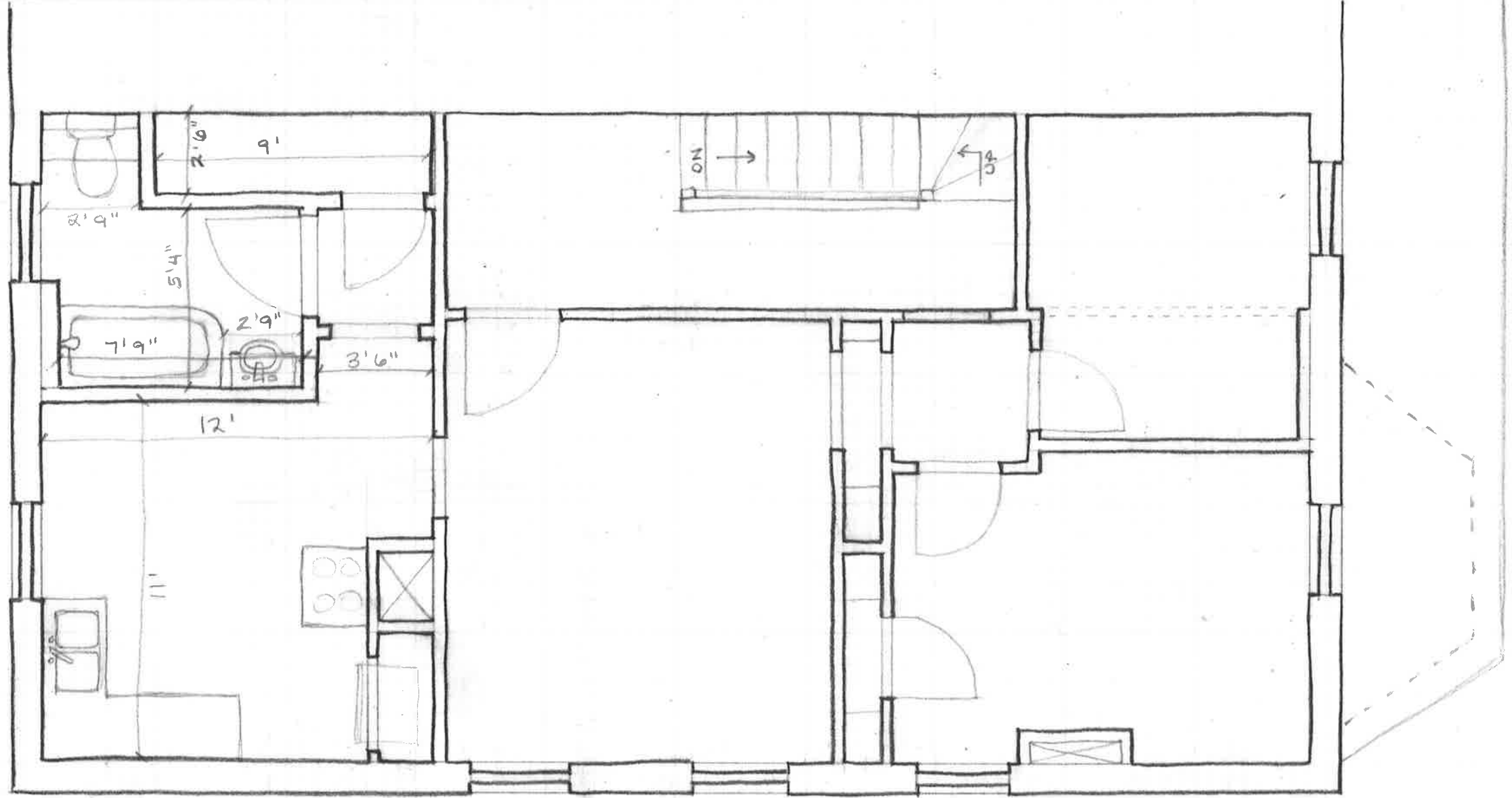
SECOND FLOOR EXISTING @ 1" = 1/4" SCALE
