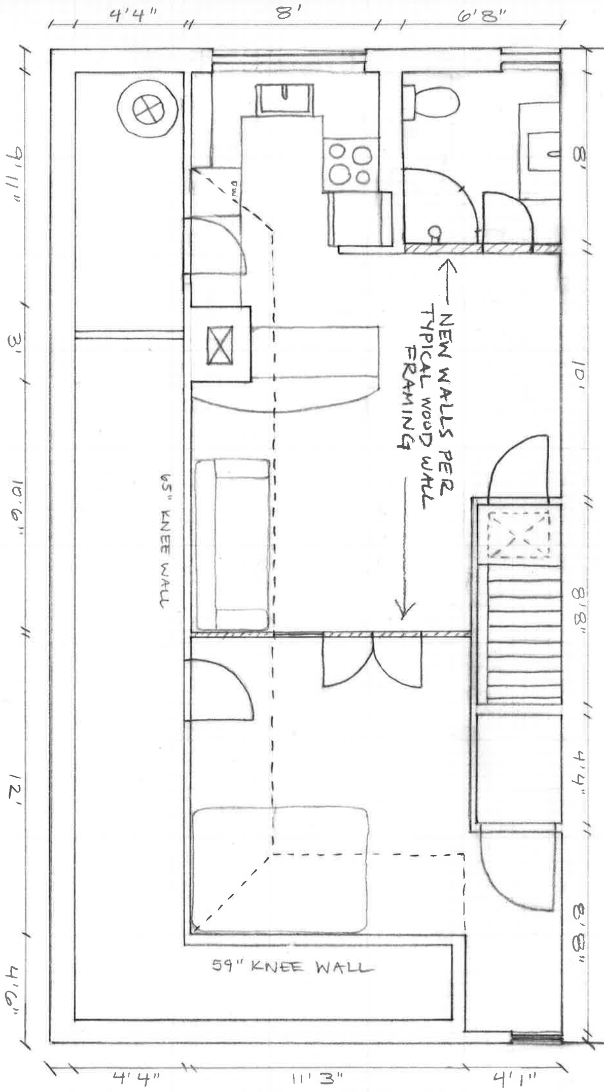
THIRD FLOOR RENOVATION PLAN @ 1" = 1/4" SCALE
