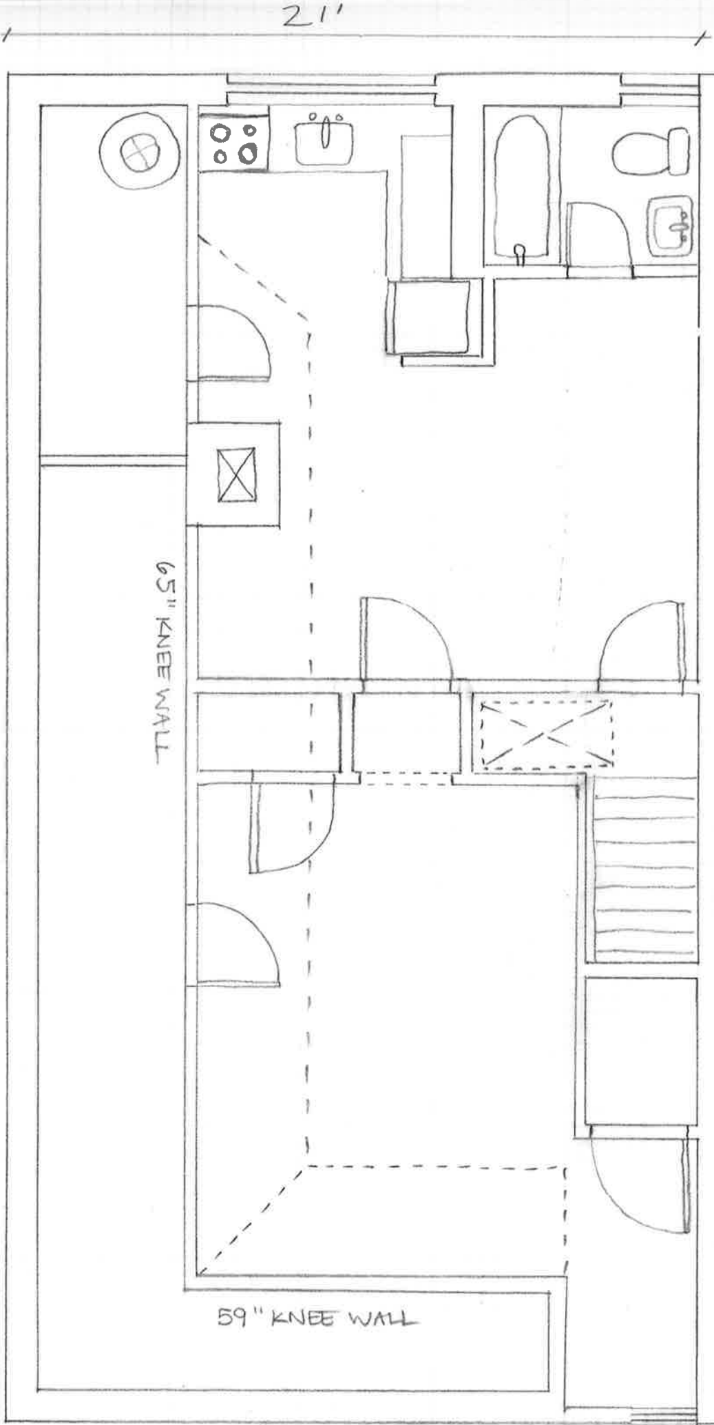
THIRD FLOOR EXISTING PLAN @ 1' = 1/4" SCALE
