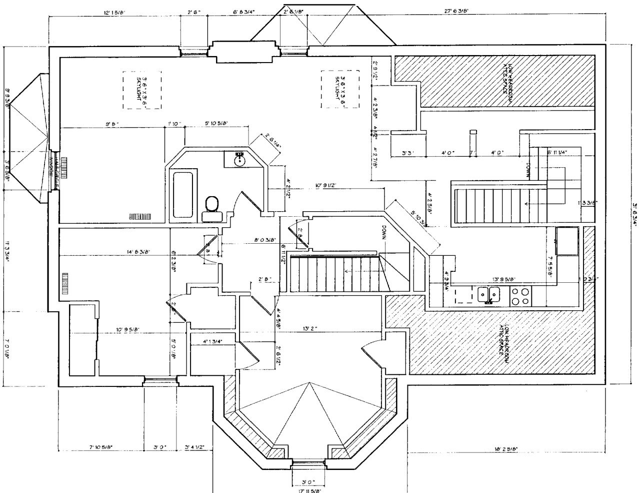
1/2" = 1' 3RD FLOOR PLAN
