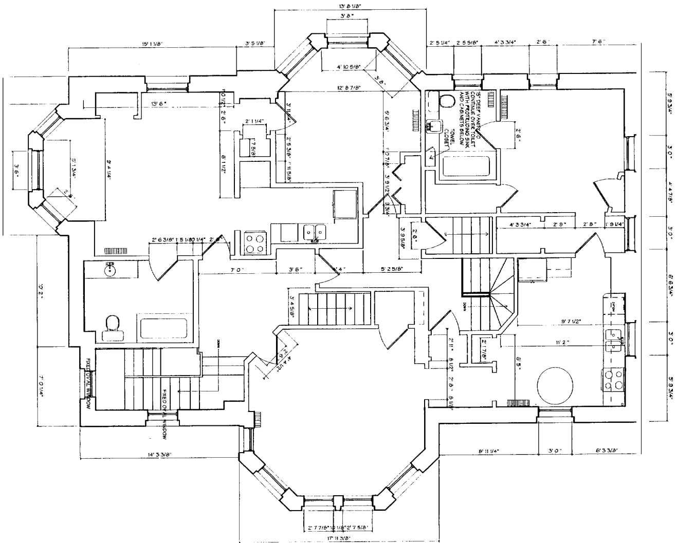
1/2" = 1' 2ND FLOOR PLAN
