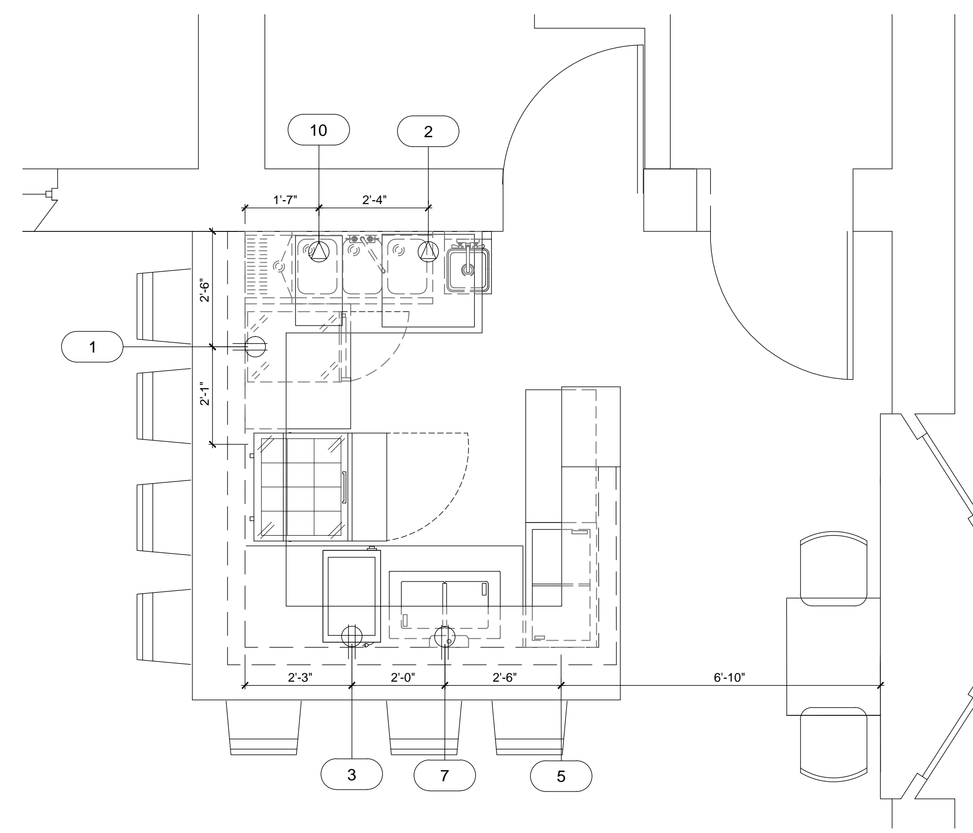
ELECTRICAL ROUGH-IN PLAN SCALE: 1/2" = 1'-0"
