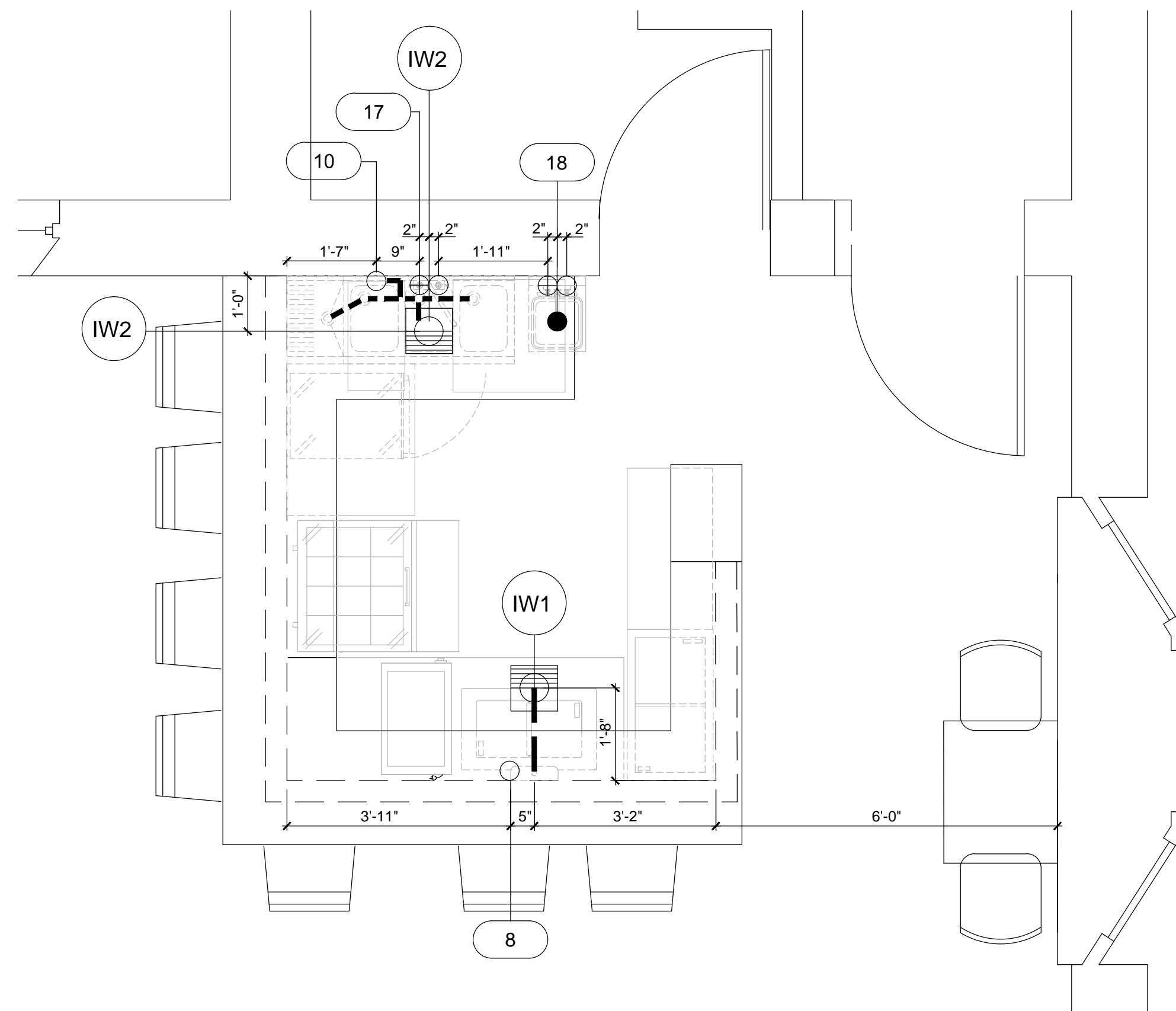
PLUMBING ROUGH-IN PLAN SCALE: 1/2" = 1'-0"
