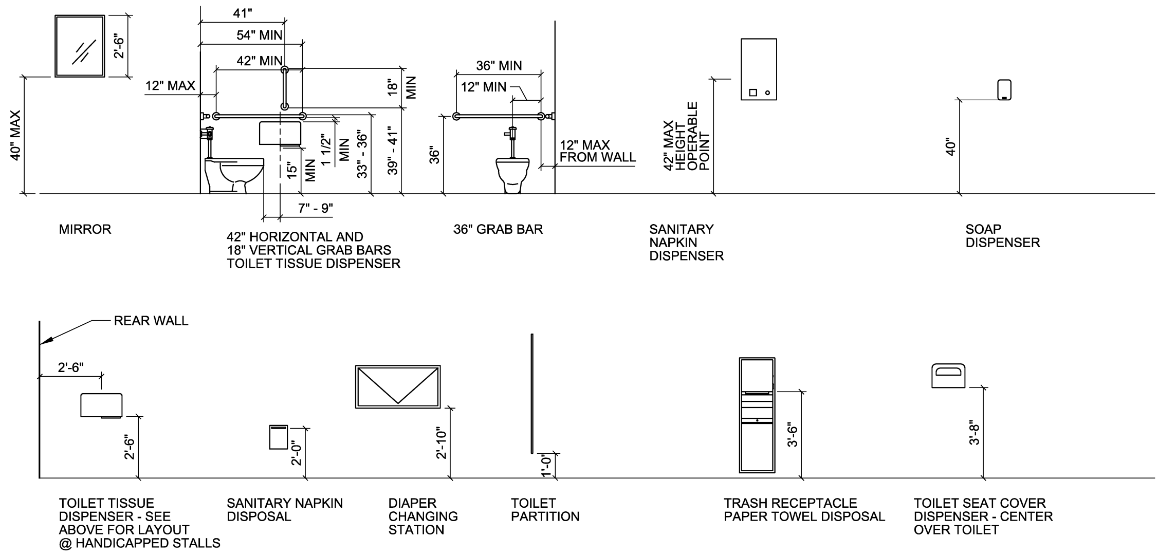
RESTROOM ACCESSORIES & MOUNTING HEIGHTS SCALE: NTS
